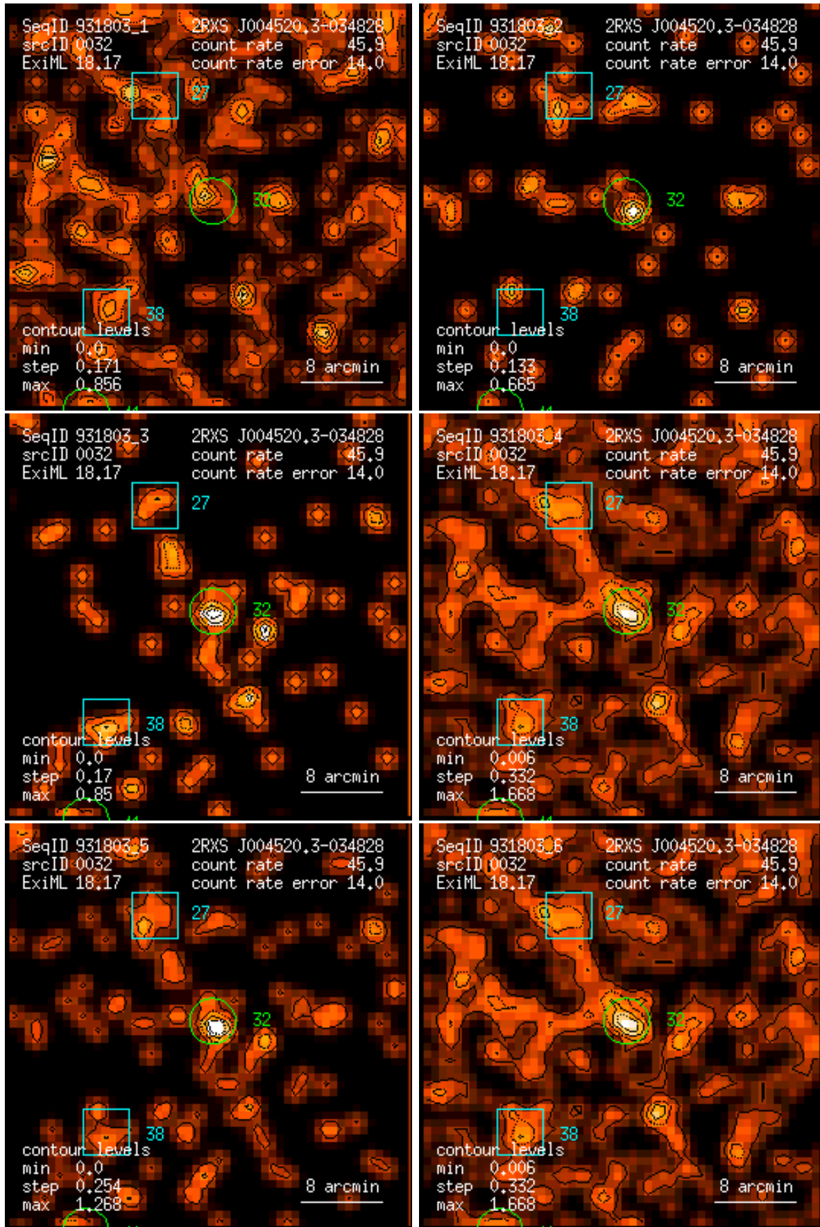
Figure 32: RASS 931803: detection 0032: band rate images, Gaussian filter: (1) PSPC channels 11 – 41, (2) 52 – 90, (3) 91 – 201, (4) 11 – 235, (5) 52 – 201, (6) 11 – 201. Broad band rates in counts/ks. Band rate contour levels in counts/ks/arcmin 2 .
