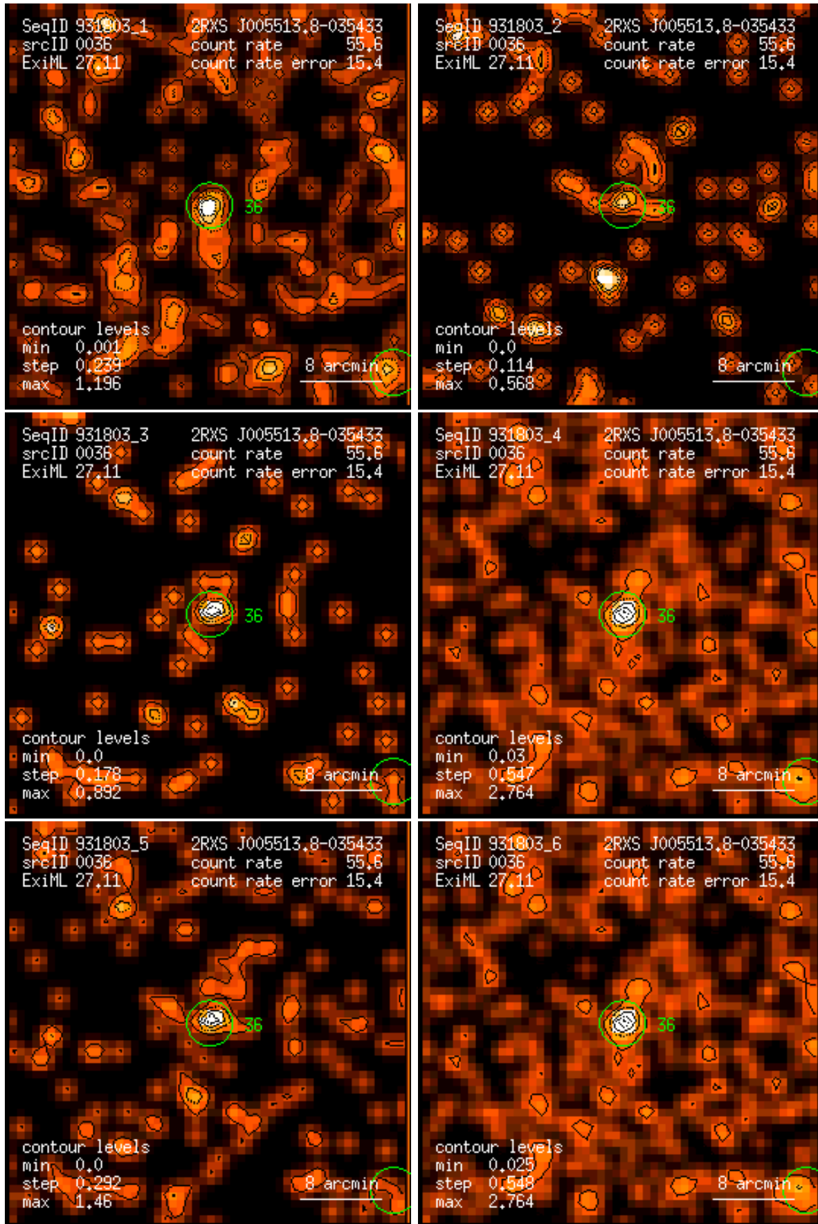
Figure 36: RASS 931803: detection 0036: band rate images, Gaussian filter: (1) PSPC channels 11 – 41, (2) 52 – 90, (3) 91 – 201, (4) 11 – 235, (5) 52 – 201, (6) 11 – 201. Broad band rates in counts/ks. Band rate contour levels in counts/ks/arcmin 2 .
