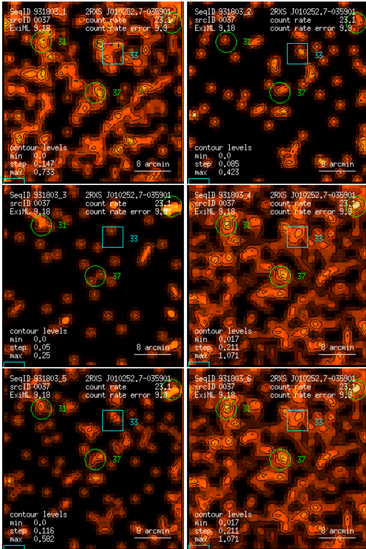
Figure 37: RASS 931803: detection 0037: band rate images, Gaussian filter: (1) PSPC channels 11 – 41, (2) 52 – 90, (3) 91 – 201, (4) 11 – 235, (5) 52 – 201, (6) 11 – 201. Broad band rates in counts/ks. Band rate contour levels in counts/ks/arcmin 2 .
