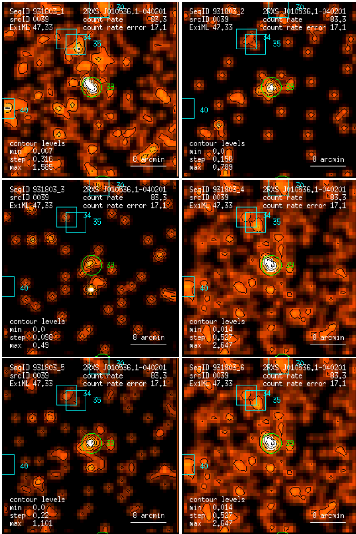
Figure 39: RASS 931803: detection 0039: band rate images, Gaussian filter: (1) PSPC channels 11 – 41, (2) 52 – 90, (3) 91 – 201, (4) 11 – 235, (5) 52 – 201, (6) 11 – 201. Broad band rates in counts/ks. Band rate contour levels in counts/ks/arcmin 2 .
