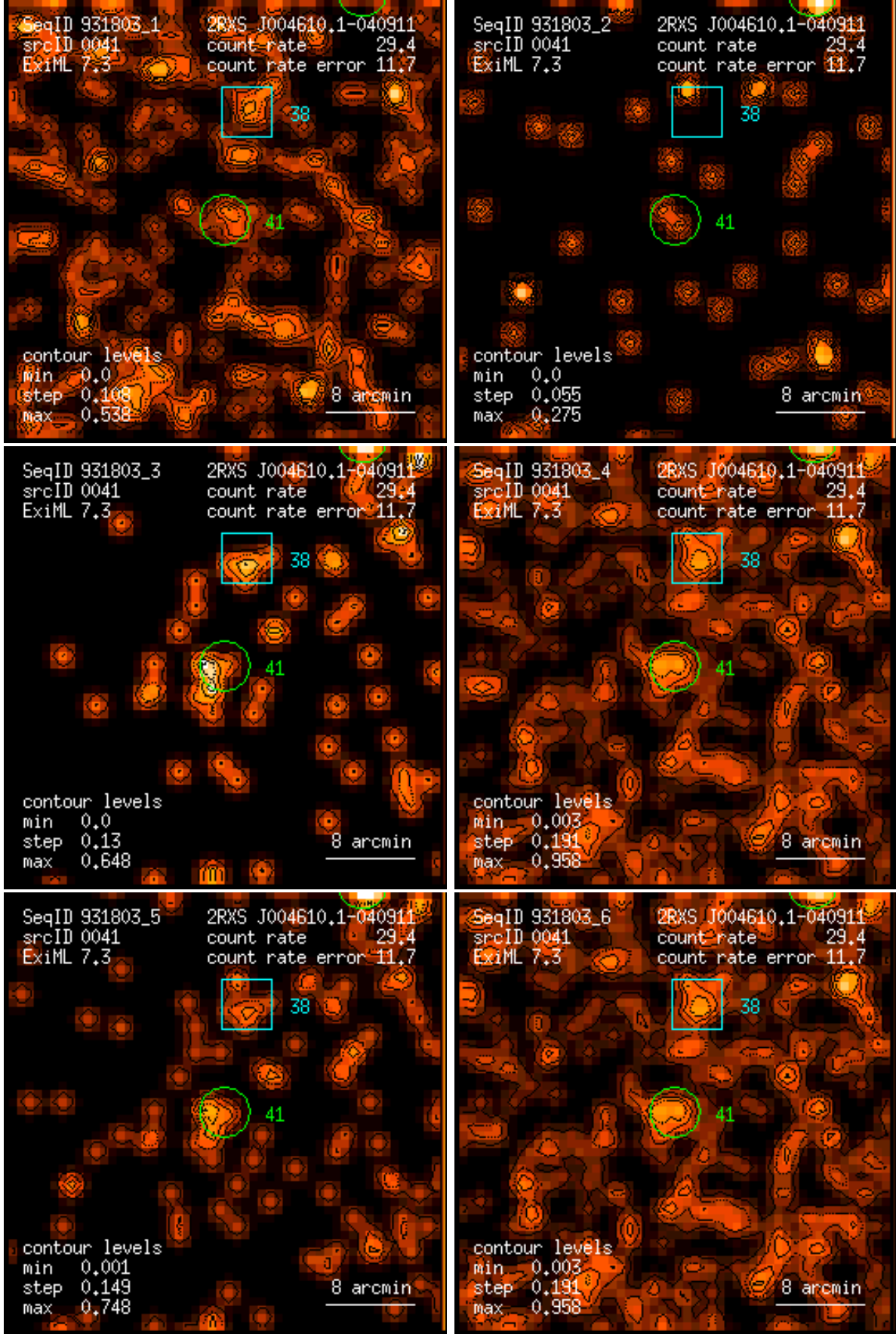
Figure 41: RASS 931803: detection 0041: band rate images, Gaussian filter: (1) PSPC channels 11 – 41, (2) 52 – 90, (3) 91 – 201, (4) 11 – 235, (5) 52 – 201, (6) 11 – 201. Broad band rates in counts/ks. Band rate contour levels in counts/ks/arcmin 2 .
