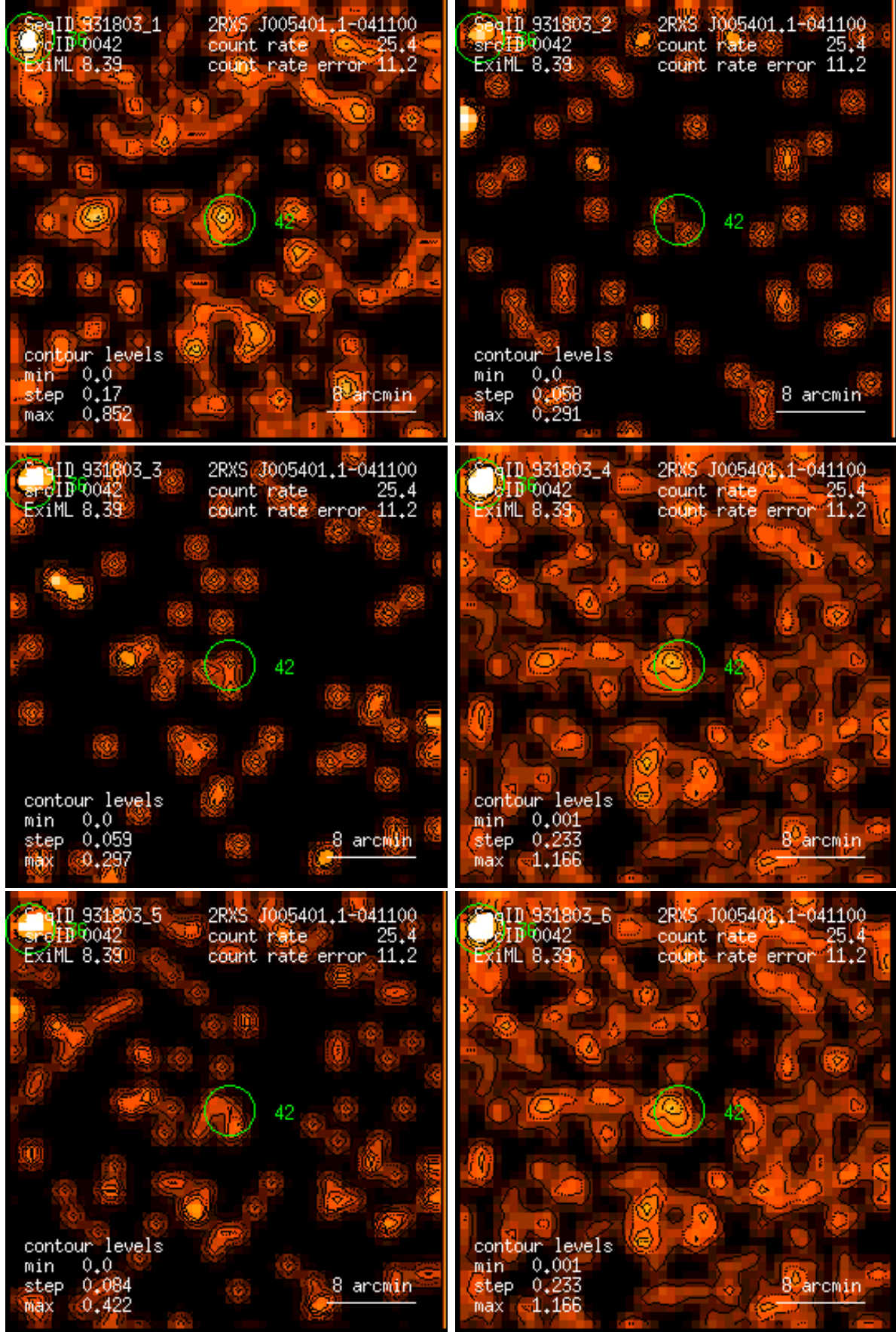
Figure 42: RASS 931803: detection 0042: band rate images, Gaussian filter: (1) PSPC channels 11 – 41, (2) 52 – 90, (3) 91 – 201, (4) 11 – 235, (5) 52 – 201, (6) 11 – 201. Broad band rates in counts/ks. Band rate contour levels in counts/ks/arcmin 2 .
