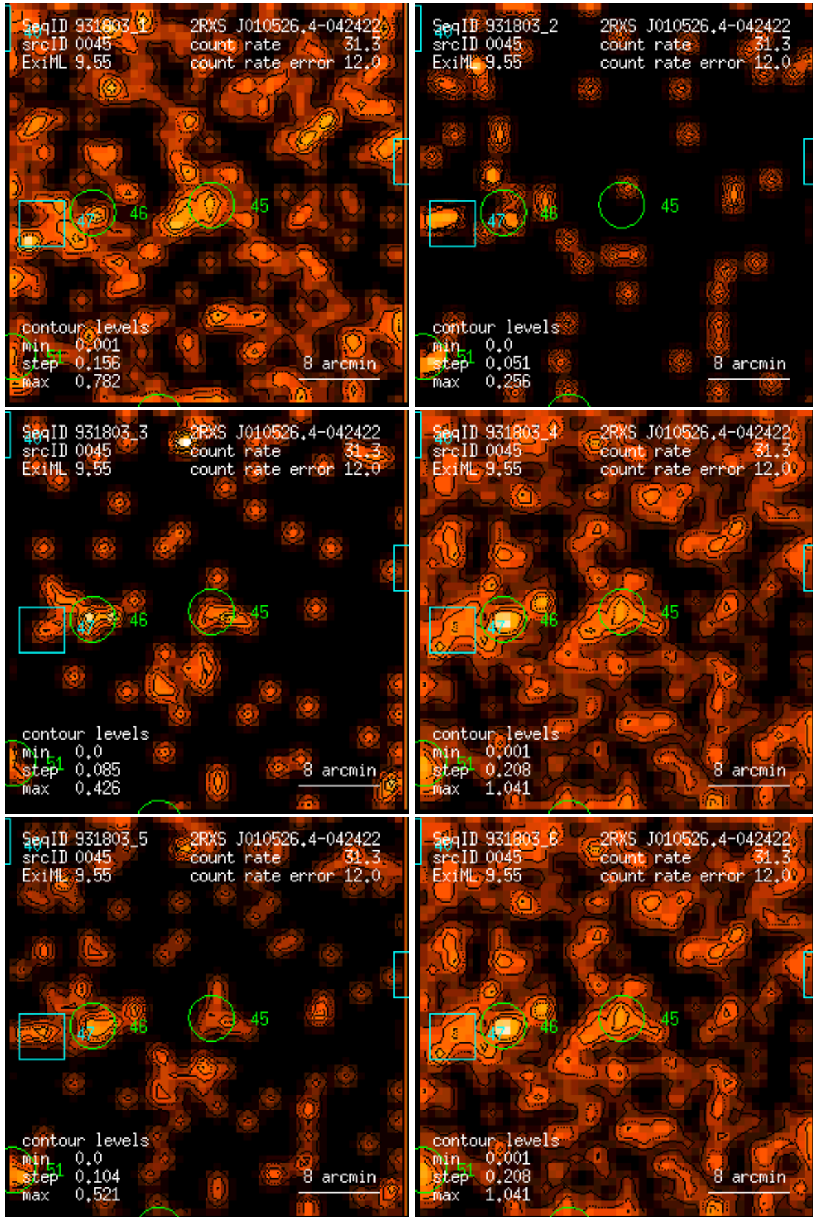
Figure 45: RASS 931803: detection 0045: band rate images, Gaussian filter: (1) PSPC channels 11 – 41, (2) 52 – 90, (3) 91 – 201, (4) 11 – 235, (5) 52 – 201, (6) 11 – 201. Broad band rates in counts/ks. Band rate contour levels in counts/ks/arcmin 2 .
