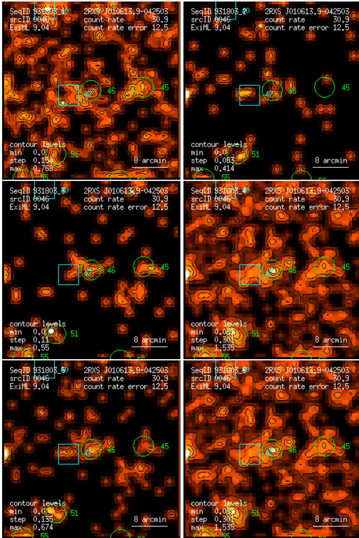
Figure 46: RASS 931803: detection 0046: band rate images, Gaussian filter: (1) PSPC channels 11 – 41, (2) 52 – 90, (3) 91 – 201, (4) 11 – 235, (5) 52 – 201, (6) 11 – 201. Broad band rates in counts/ks. Band rate contour levels in counts/ks/arcmin 2 .
