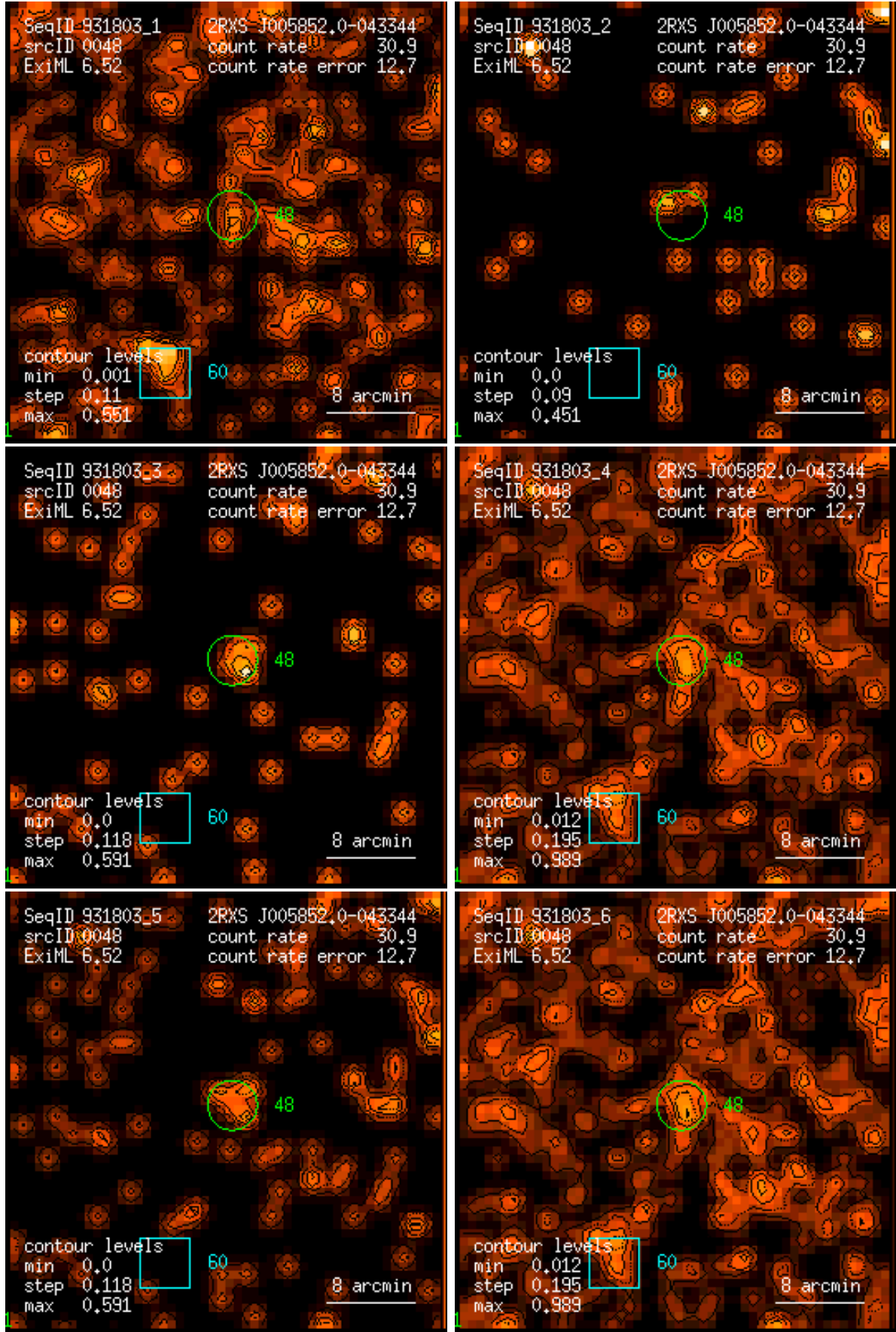
Figure 48: RASS 931803: detection 0048: band rate images, Gaussian filter: (1) PSPC channels 11 – 41, (2) 52 – 90, (3) 91 – 201, (4) 11 – 235, (5) 52 – 201, (6) 11 – 201. Broad band rates in counts/ks. Band rate contour levels in counts/ks/arcmin 2 .
