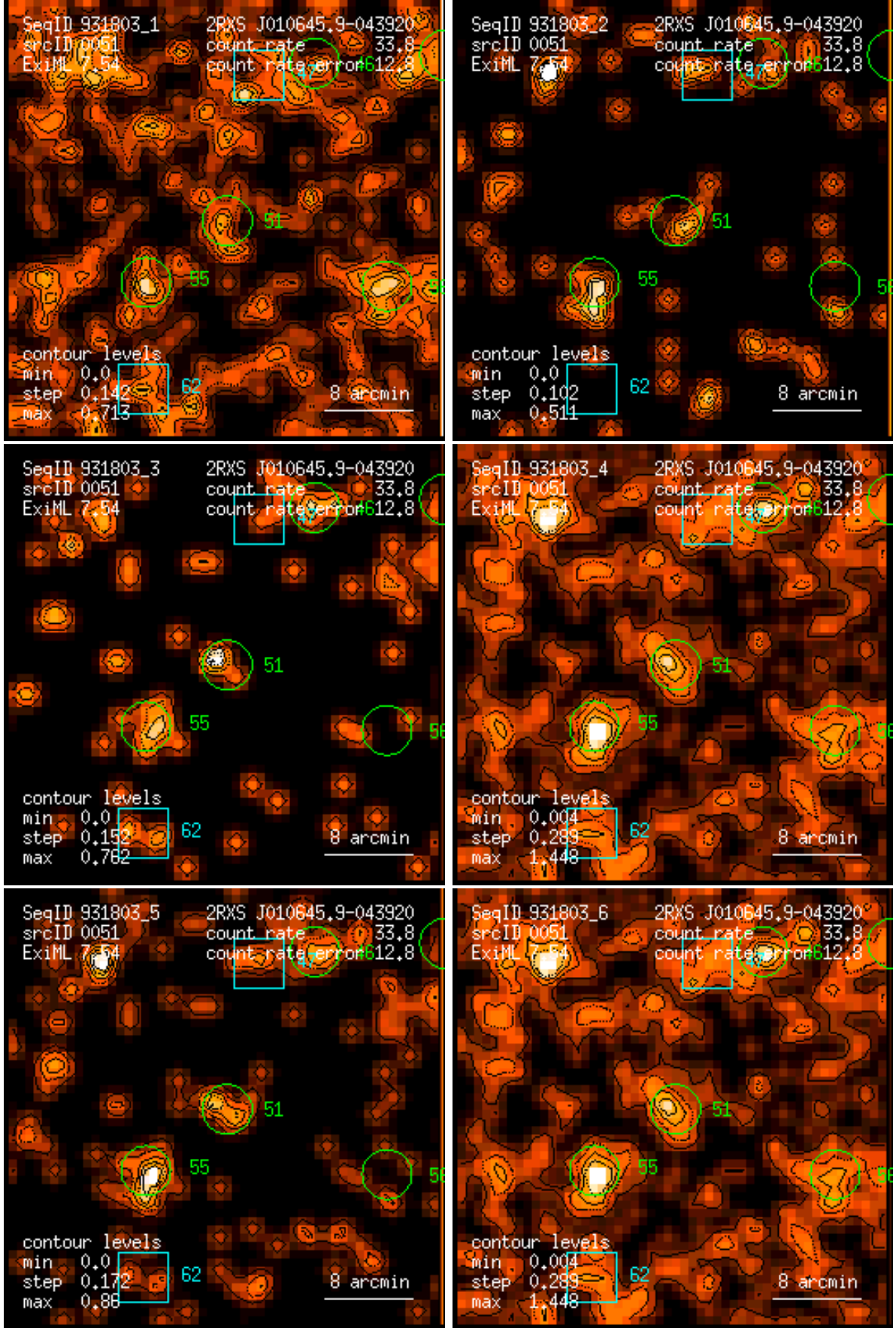
Figure 51: RASS 931803: detection 0051: band rate images, Gaussian filter: (1) PSPC channels 11 – 41, (2) 52 – 90, (3) 91 – 201, (4) 11 – 235, (5) 52 – 201, (6) 11 – 201. Broad band rates in counts/ks. Band rate contour levels in counts/ks/arcmin 2 .
