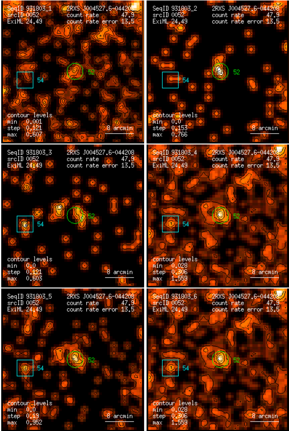
Figure 52: RASS 931803: detection 0052: band rate images, Gaussian filter: (1) PSPC channels 11 – 41, (2) 52 – 90, (3) 91 – 201, (4) 11 – 235, (5) 52 – 201, (6) 11 – 201. Broad band rates in counts/ks. Band rate contour levels in counts/ks/arcmin 2 .
