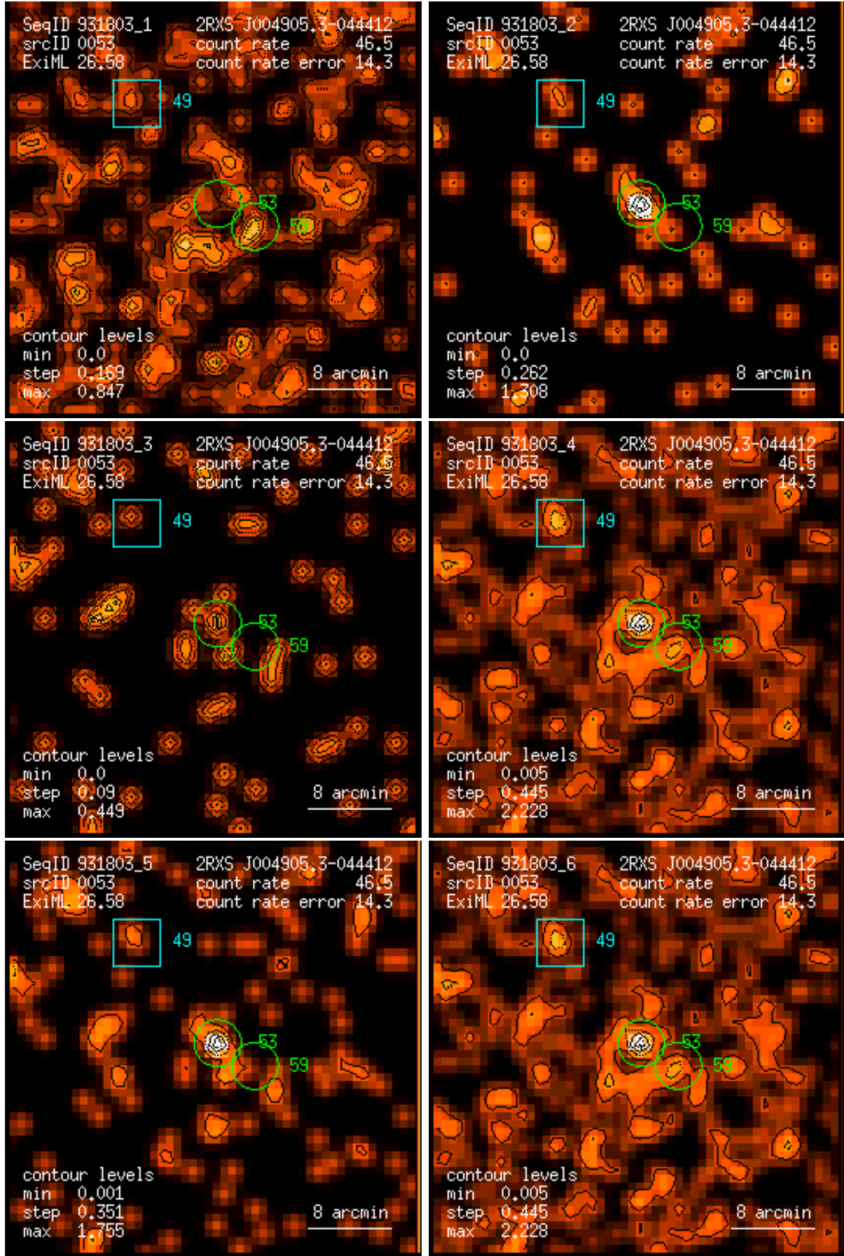
Figure 53: RASS 931803: detection 0053: band rate images, Gaussian filter: (1) PSPC channels 11 – 41, (2) 52 – 90, (3) 91 – 201, (4) 11 – 235, (5) 52 – 201, (6) 11 – 201. Broad band rates in counts/ks. Band rate contour levels in counts/ks/arcmin 2 .
