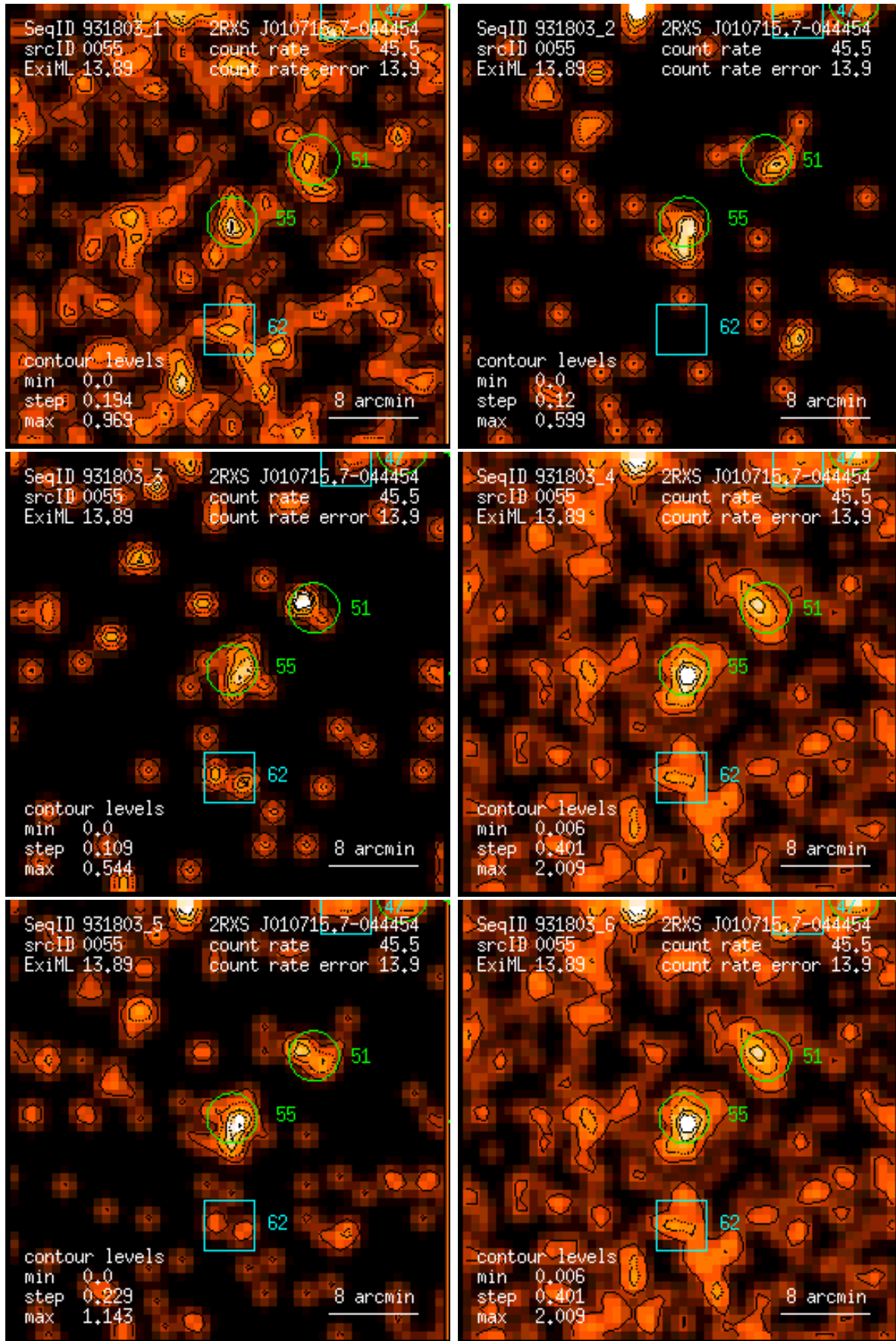
Figure 55: RASS 931803: detection 0055: band rate images, Gaussian filter: (1) PSPC channels 11 – 41, (2) 52 – 90, (3) 91 – 201, (4) 11 – 235, (5) 52 – 201, (6) 11 – 201. Broad band rates in counts/ks. Band rate contour levels in counts/ks/arcmin 2 .
