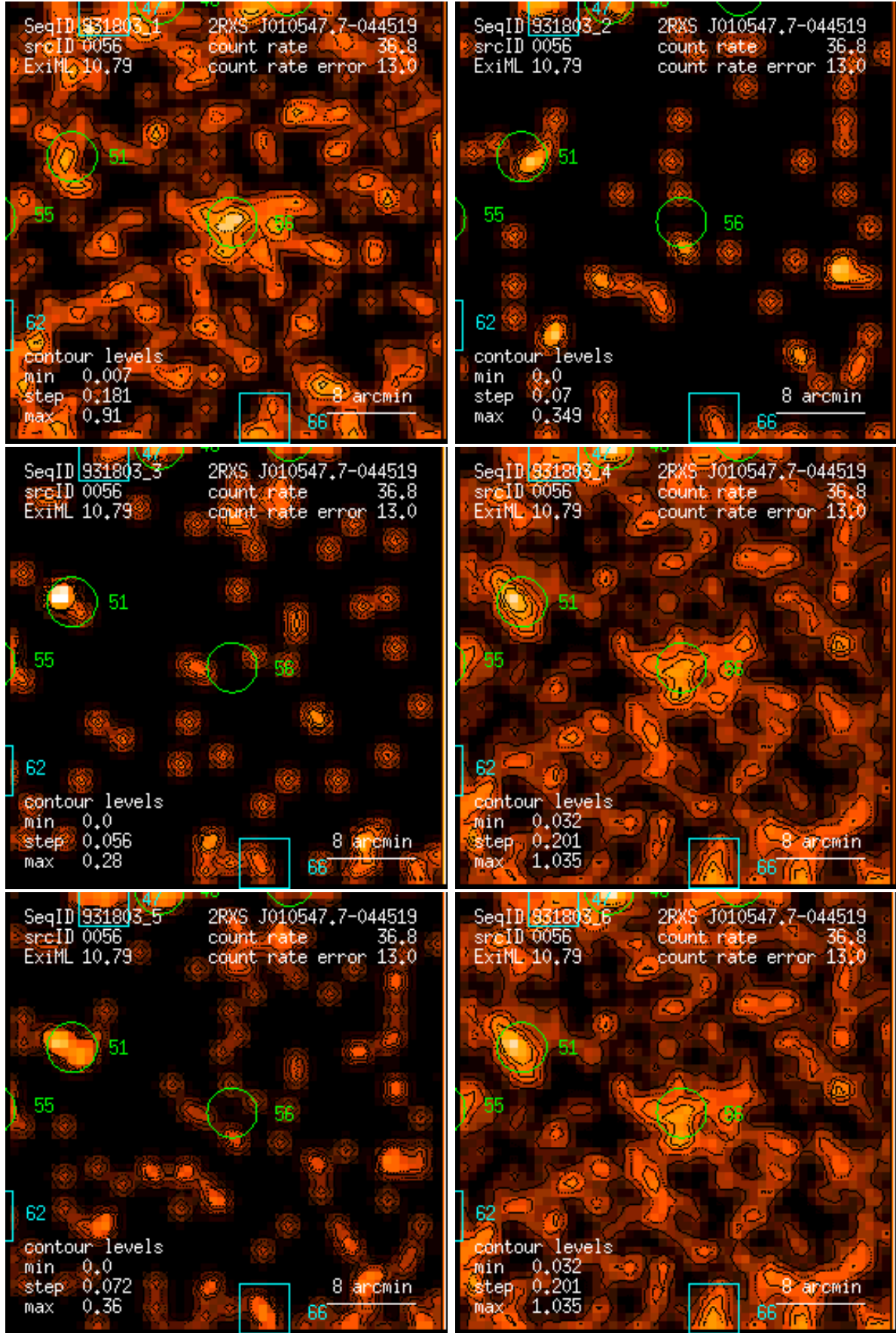
Figure 56: RASS 931803: detection 0056: band rate images, Gaussian filter: (1) PSPC channels 11 – 41, (2) 52 – 90, (3) 91 – 201, (4) 11 – 235, (5) 52 – 201, (6) 11 – 201. Broad band rates in counts/ks. Band rate contour levels in counts/ks/arcmin 2 .
