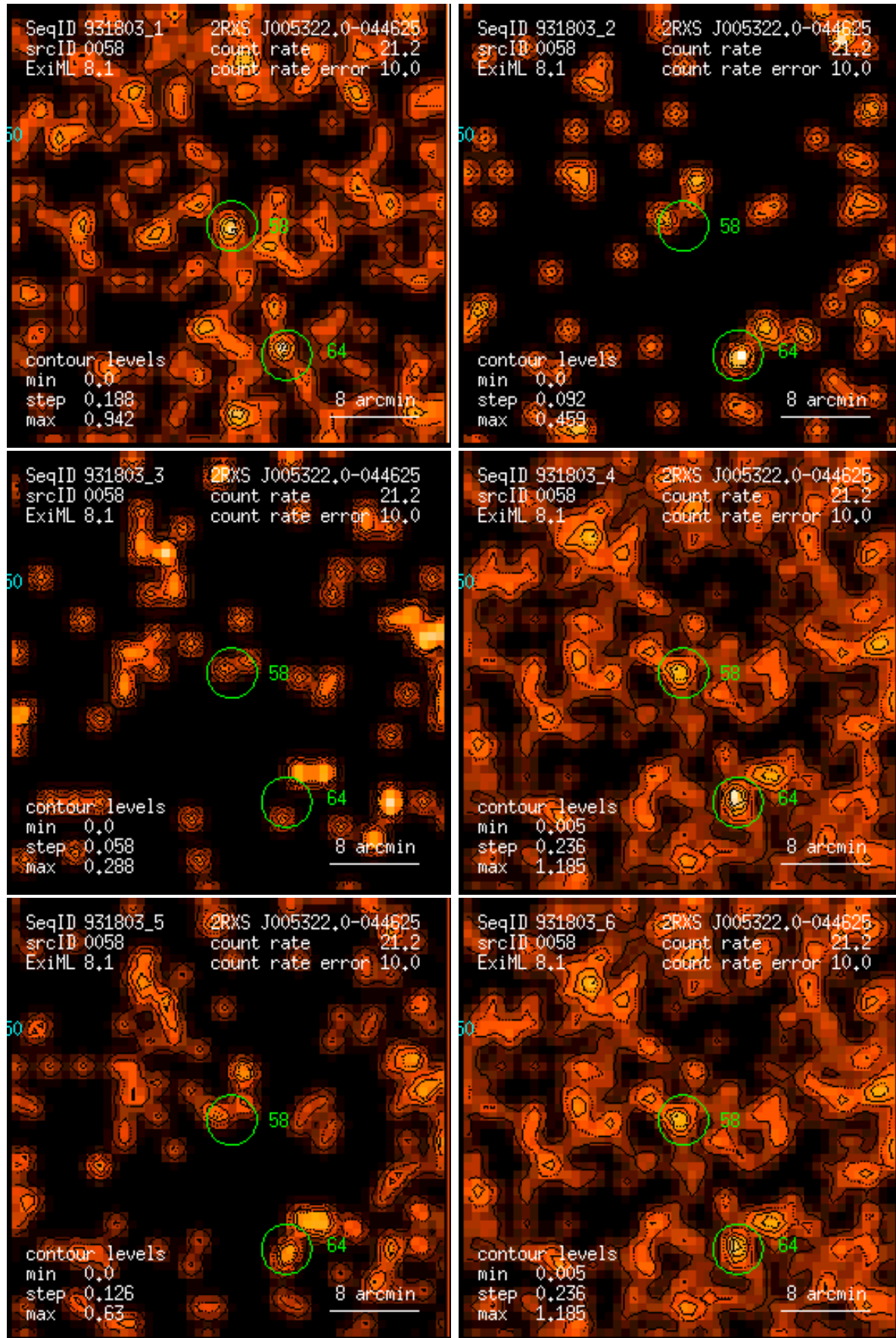
Figure 58: RASS 931803: detection 0058: band rate images, Gaussian filter: (1) PSPC channels 11 – 41, (2) 52 – 90, (3) 91 – 201, (4) 11 – 235, (5) 52 – 201, (6) 11 – 201. Broad band rates in counts/ks. Band rate contour levels in counts/ks/arcmin 2 .
