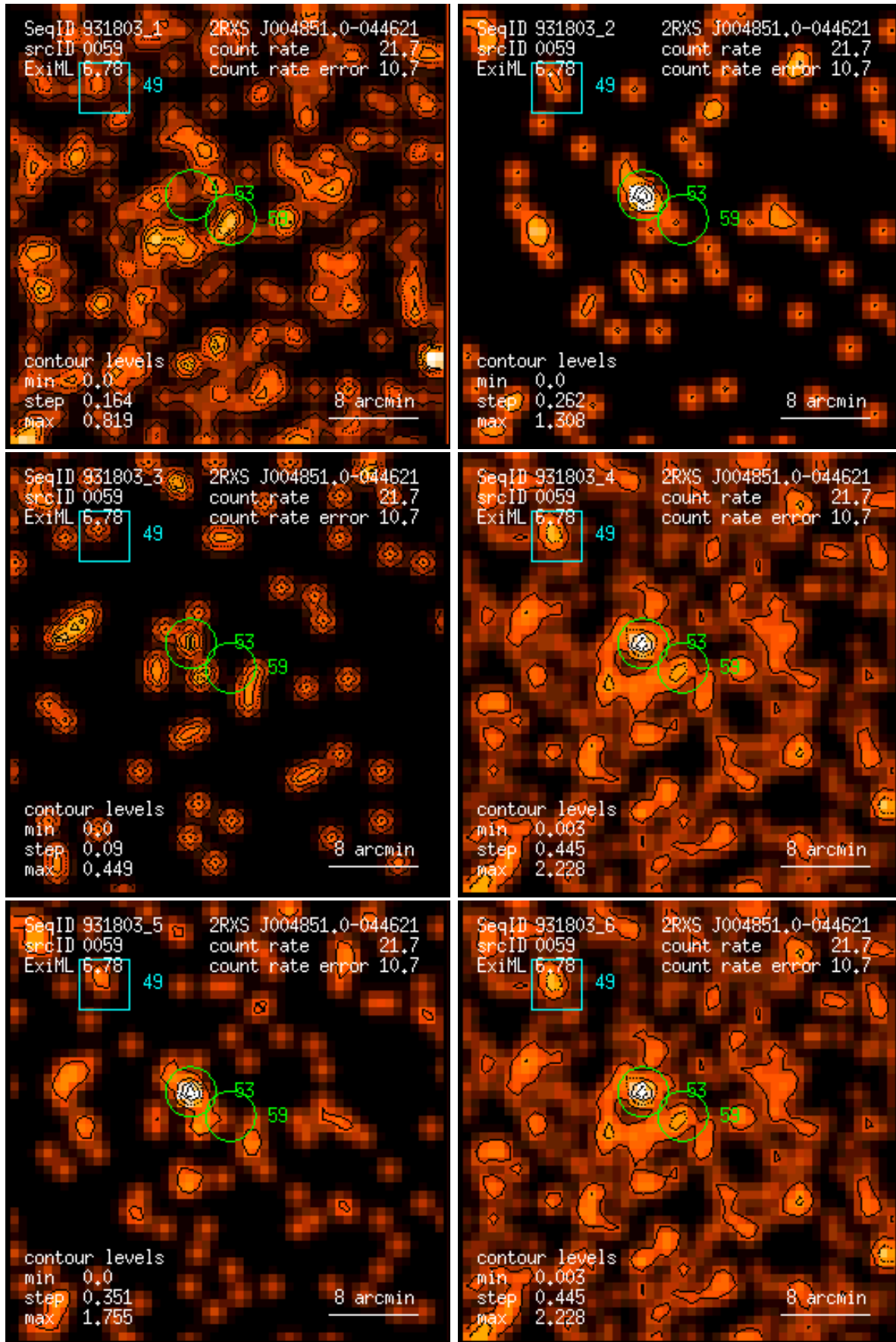
Figure 59: RASS 931803: detection 0059: band rate images, Gaussian filter: (1) PSPC channels 11 – 41, (2) 52 – 90, (3) 91 – 201, (4) 11 – 235, (5) 52 – 201, (6) 11 – 201. Broad band rates in counts/ks. Band rate contour levels in counts/ks/arcmin 2 .
