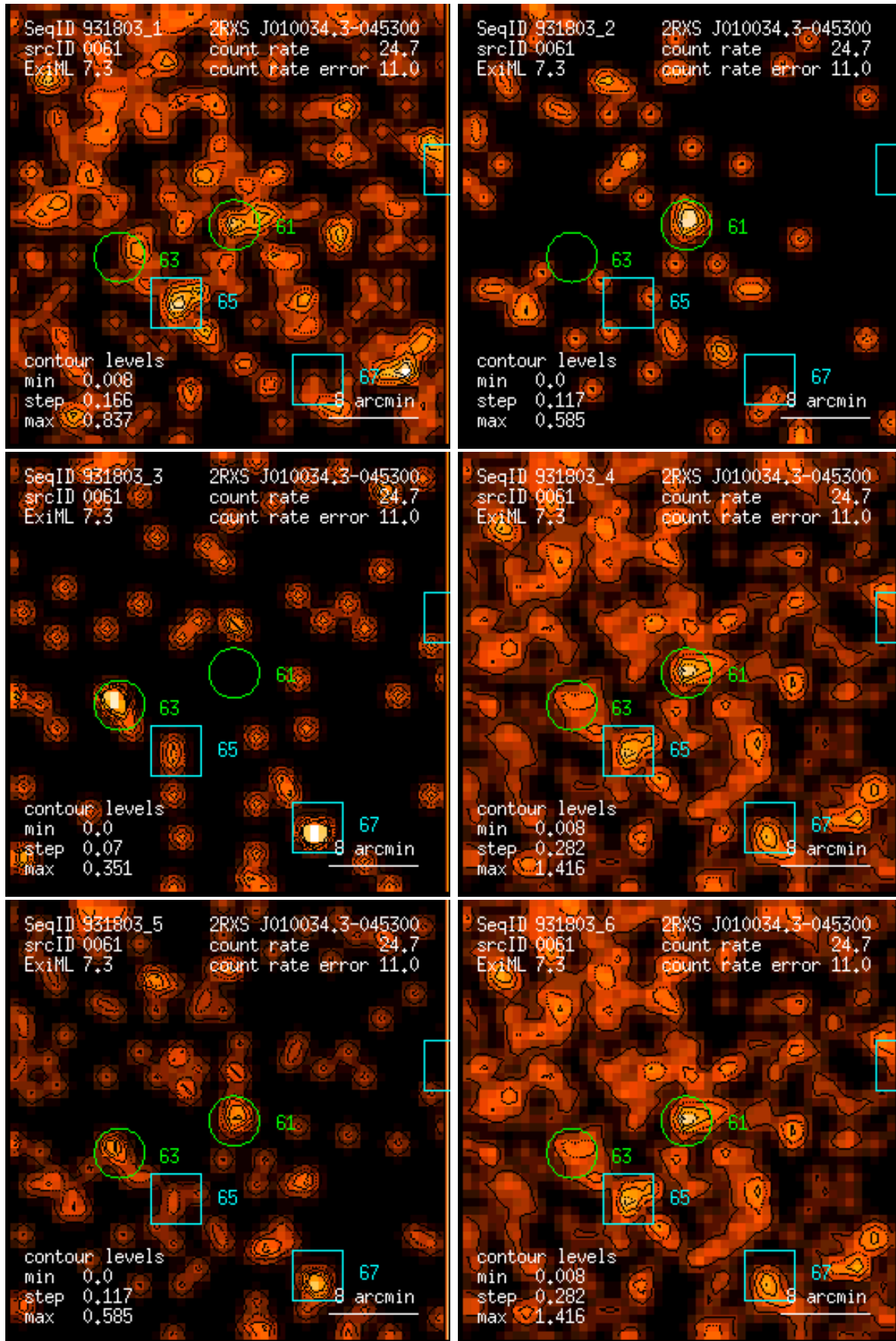
Figure 61: RASS 931803: detection 0061: band rate images, Gaussian filter: (1) PSPC channels 11 – 41, (2) 52 – 90, (3) 91 – 201, (4) 11 – 235, (5) 52 – 201, (6) 11 – 201. Broad band rates in counts/ks. Band rate contour levels in counts/ks/arcmin 2 .
