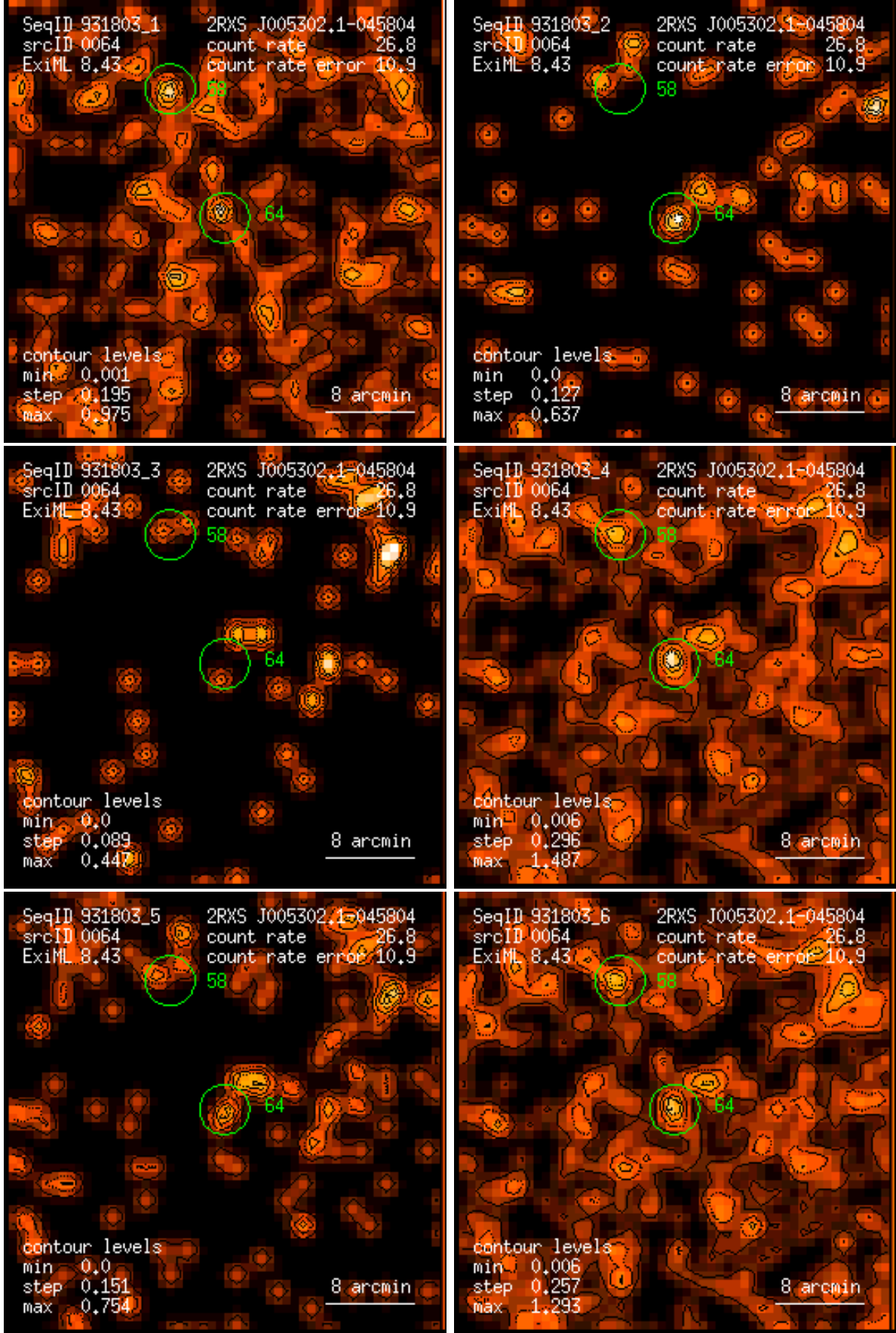
Figure 64: RASS 931803: detection 0064: band rate images, Gaussian filter: (1) PSPC channels 11 – 41, (2) 52 – 90, (3) 91 – 201, (4) 11 – 235, (5) 52 – 201, (6) 11 – 201. Broad band rates in counts/ks. Band rate contour levels in counts/ks/arcmin 2 .
