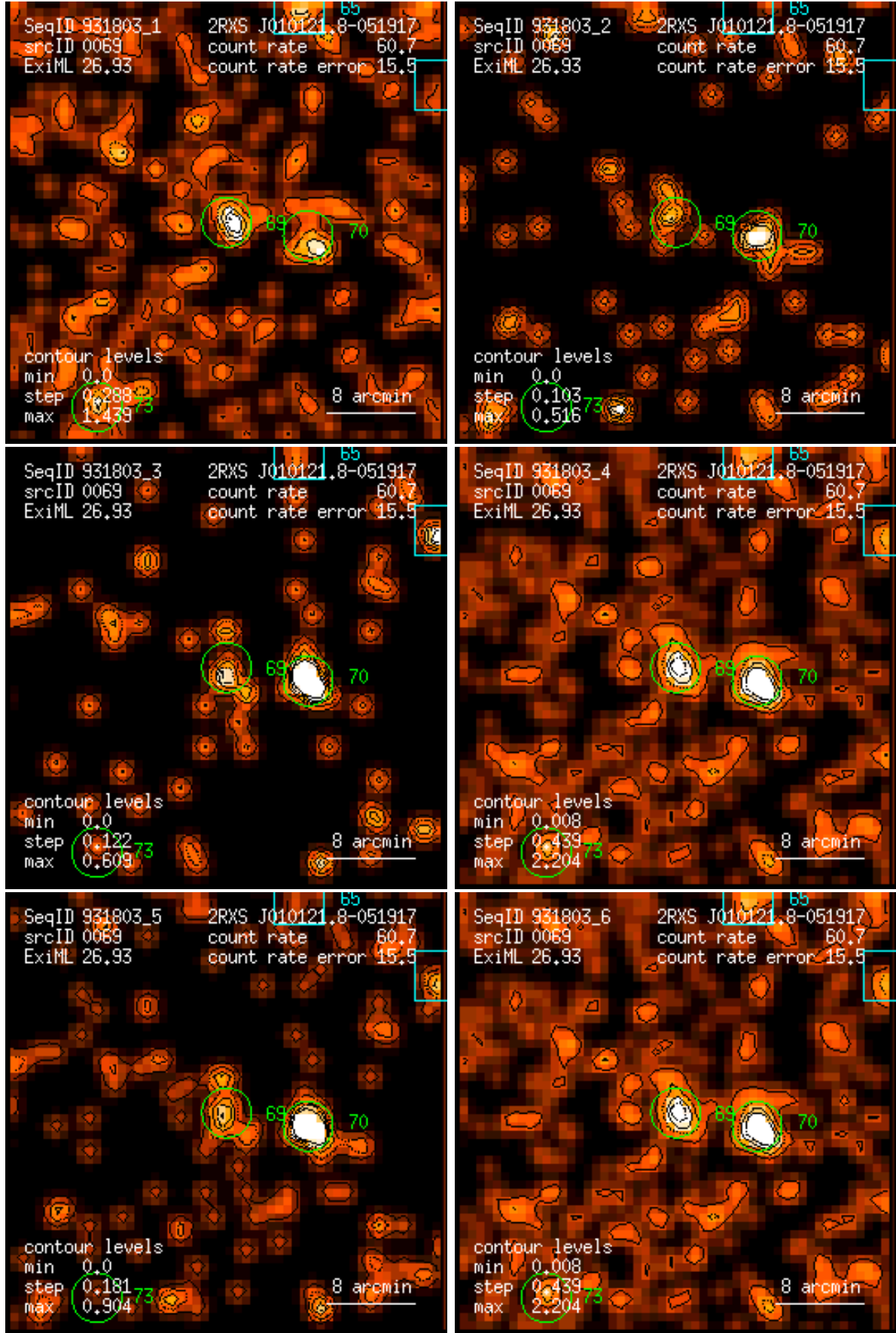
Figure 69: RASS 931803: detection 0069: band rate images, Gaussian filter: (1) PSPC channels 11 – 41, (2) 52 – 90, (3) 91 – 201, (4) 11 – 235, (5) 52 – 201, (6) 11 – 201. Broad band rates in counts/ks. Band rate contour levels in counts/ks/arcmin 2 .
