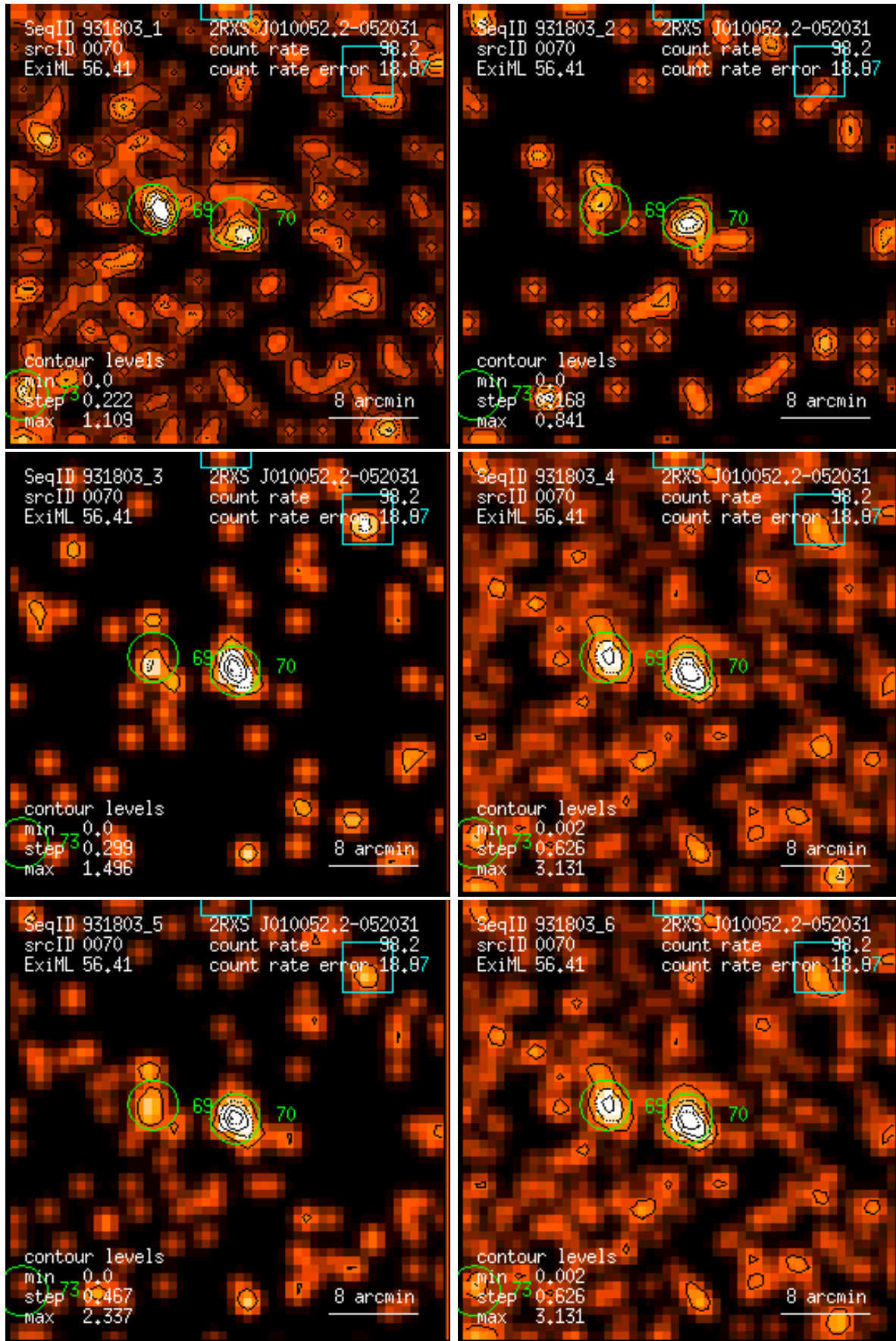
Figure 70: RASS 931803: detection 0070: band rate images, Gaussian filter: (1) PSPC channels 11 – 41, (2) 52 – 90, (3) 91 – 201, (4) 11 – 235, (5) 52 – 201, (6) 11 – 201. Broad band rates in counts/ks. Band rate contour levels in counts/ks/arcmin 2 .
