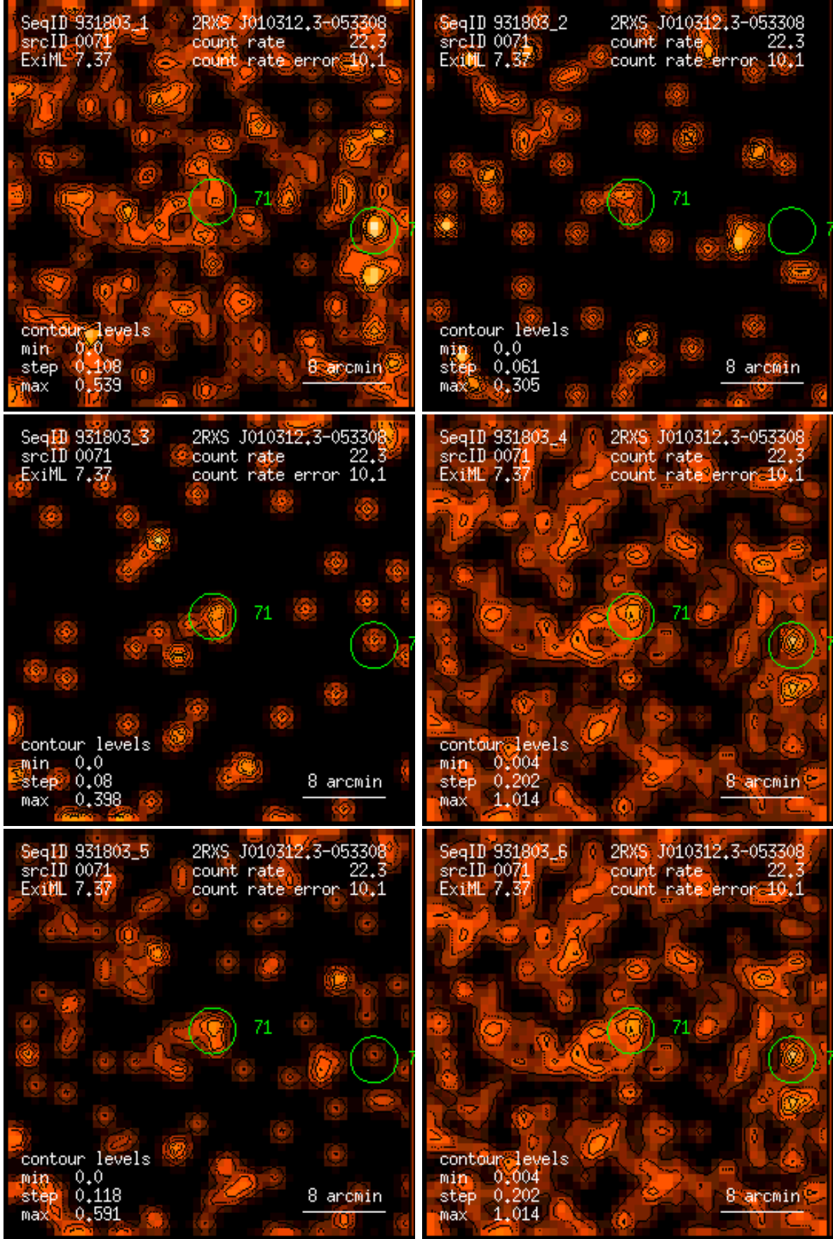
Figure 71: RASS 931803: detection 0071: band rate images, Gaussian filter: (1) PSPC channels 11 – 41, (2) 52 – 90, (3) 91 – 201, (4) 11 – 235, (5) 52 – 201, (6) 11 – 201. Broad band rates in counts/ks. Band rate contour levels in counts/ks/arcmin 2 .
