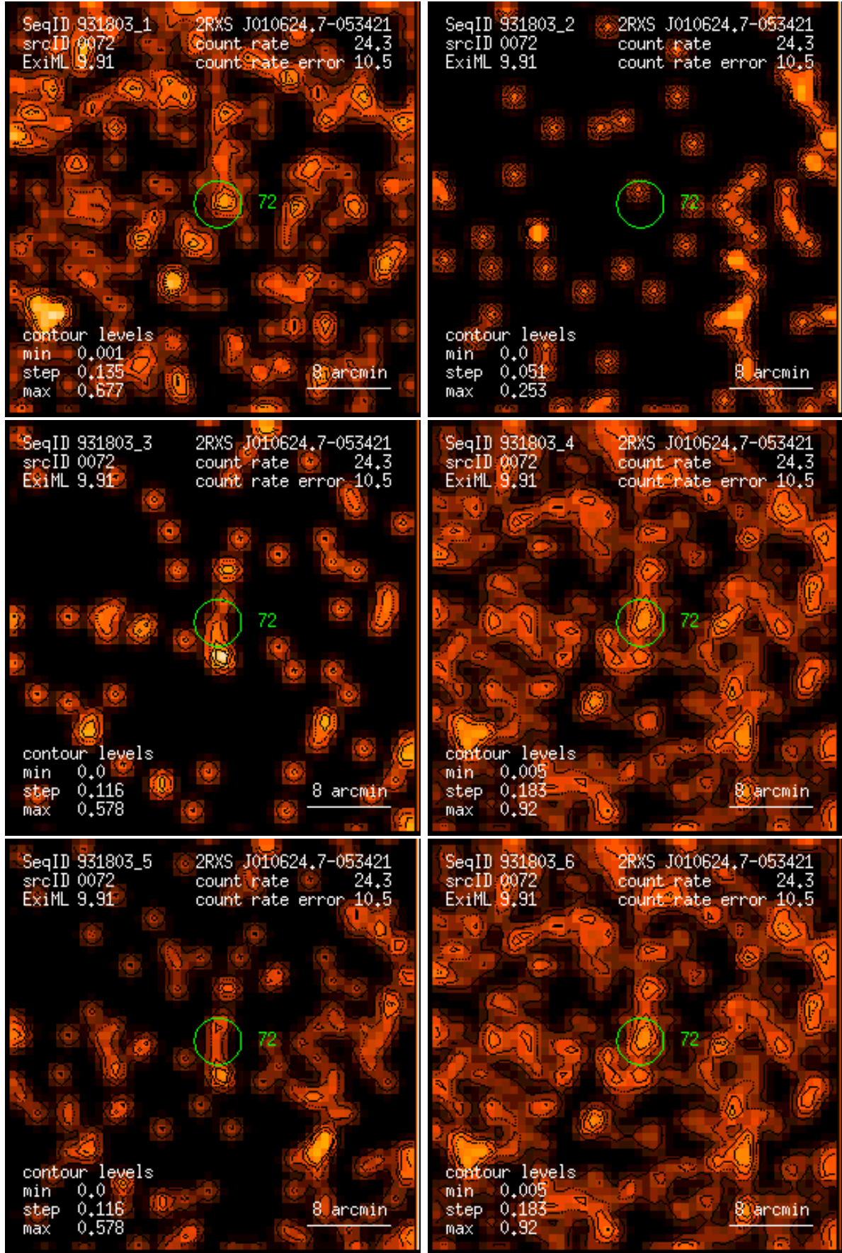
Figure 72: RASS 931803: detection 0072: band rate images, Gaussian filter: (1) PSPC channels 11 – 41, (2) 52 – 90, (3) 91 – 201, (4) 11 – 235, (5) 52 – 201, (6) 11 – 201. Broad band rates in counts/ks. Band rate contour levels in counts/ks/arcmin 2 .
