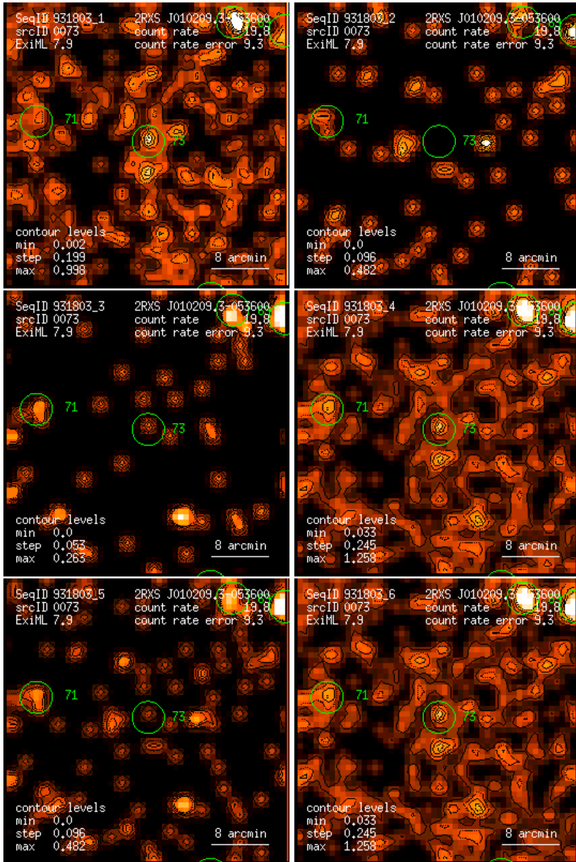
Figure 73: RASS 931803: detection 0073: band rate images, Gaussian filter: (1) PSPC channels 11 – 41, (2) 52 – 90, (3) 91 – 201, (4) 11 – 235, (5) 52 – 201, (6) 11 – 201. Broad band rates in counts/ks. Band rate contour levels in counts/ks/arcmin 2 .
