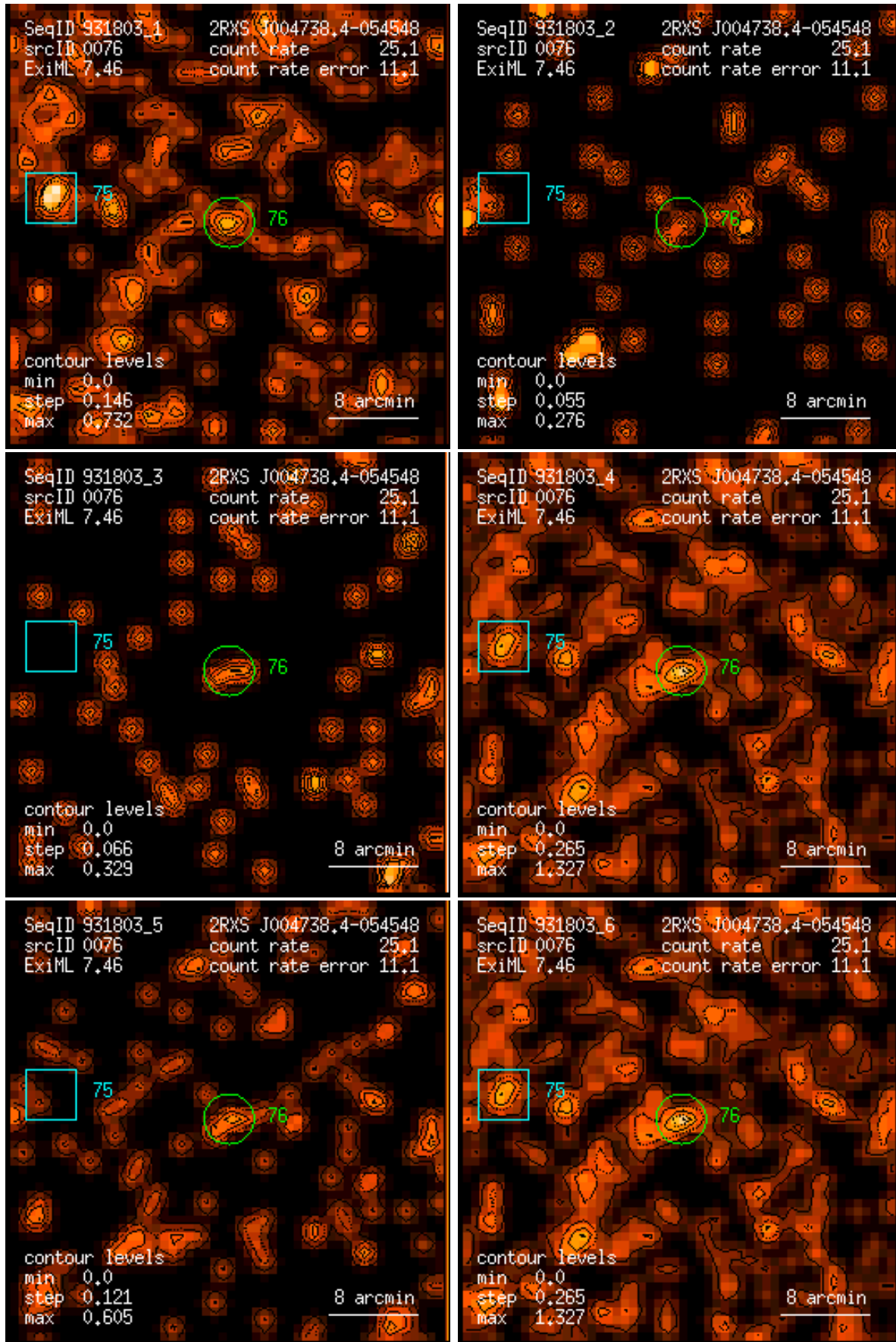
Figure 76: RASS 931803: detection 0076: band rate images, Gaussian filter: (1) PSPC channels 11 – 41, (2) 52 – 90, (3) 91 – 201, (4) 11 – 235, (5) 52 – 201, (6) 11 – 201. Broad band rates in counts/ks. Band rate contour levels in counts/ks/arcmin 2 .
