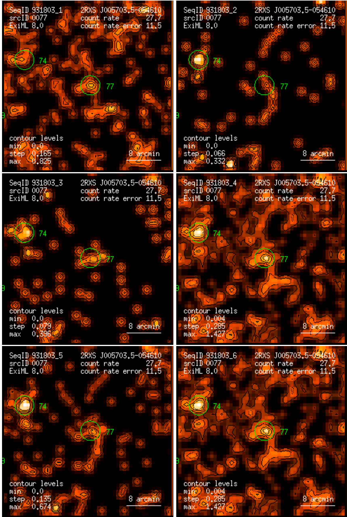
Figure 77: RASS 931803: detection 0077: band rate images, Gaussian filter: (1) PSPC channels 11 – 41, (2) 52 – 90, (3) 91 – 201, (4) 11 – 235, (5) 52 – 201, (6) 11 – 201. Broad band rates in counts/ks. Band rate contour levels in counts/ks/arcmin 2 .
