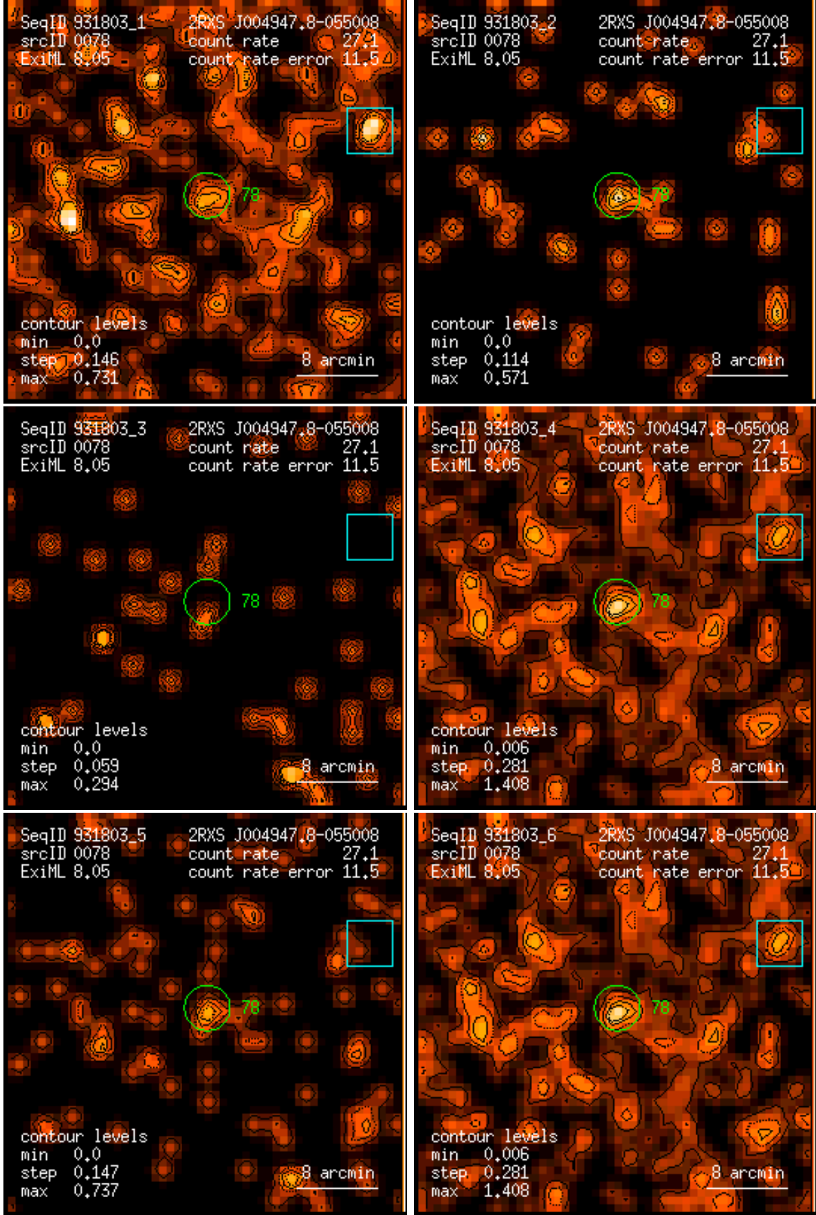
Figure 78: RASS 931803: detection 0078: band rate images, Gaussian filter: (1) PSPC channels 11 – 41, (2) 52 – 90, (3) 91 – 201, (4) 11 – 235, (5) 52 – 201, (6) 11 – 201. Broad band rates in counts/ks. Band rate contour levels in counts/ks/arcmin 2 .
