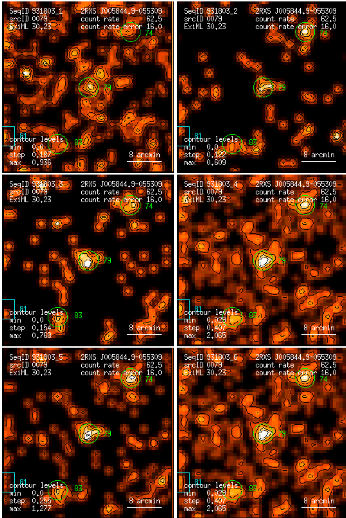
Figure 79: RASS 931803: detection 0079: band rate images, Gaussian filter: (1) PSPC channels 11 – 41, (2) 52 – 90, (3) 91 – 201, (4) 11 – 235, (5) 52 – 201, (6) 11 – 201. Broad band rates in counts/ks. Band rate contour levels in counts/ks/arcmin 2 .
