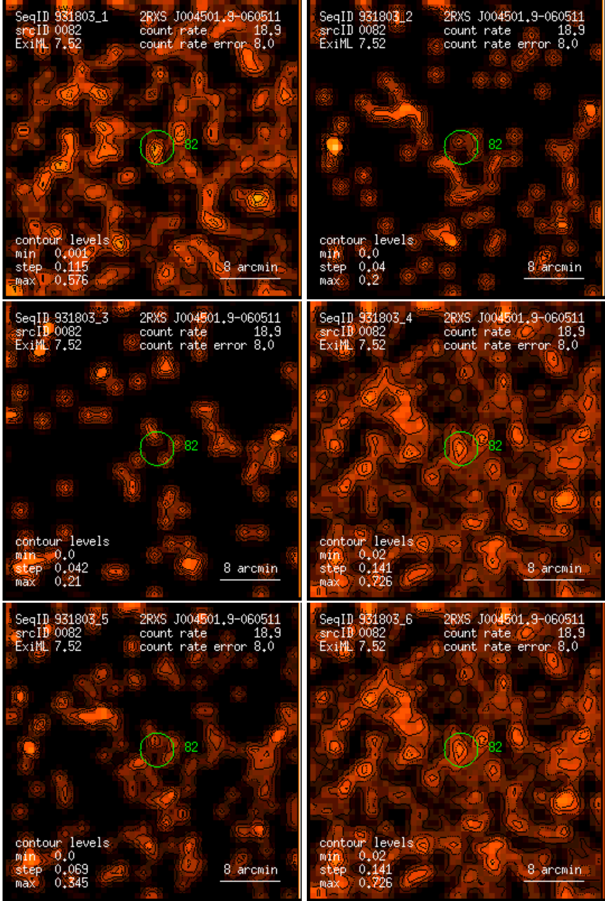
Figure 82: RASS 931803: detection 0082: band rate images, Gaussian filter: (1) PSPC channels 11 – 41, (2) 52 – 90, (3) 91 – 201, (4) 11 – 235, (5) 52 – 201, (6) 11 – 201. Broad band rates in counts/ks. Band rate contour levels in counts/ks/arcmin 2 .
