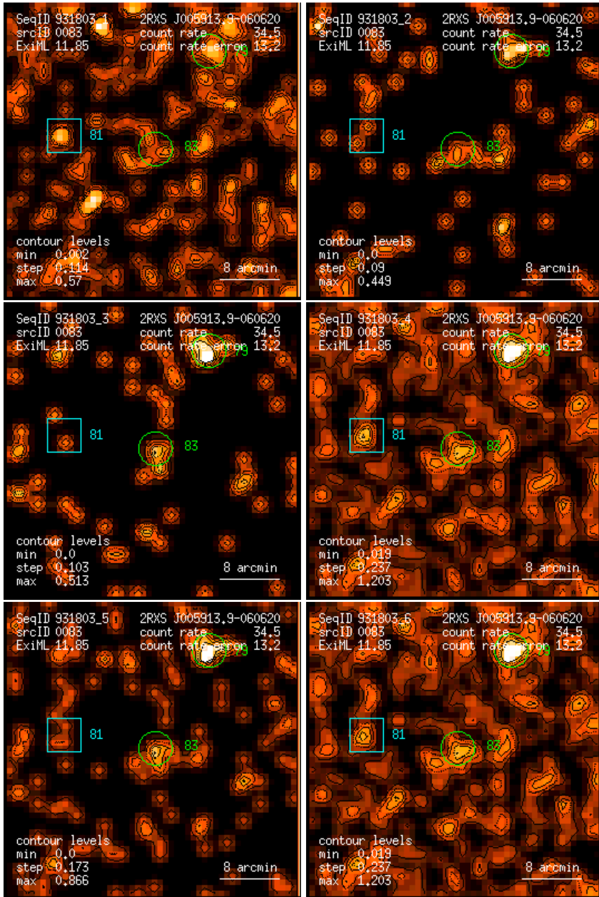
Figure 83: RASS 931803: detection 0083: band rate images, Gaussian filter: (1) PSPC channels 11 – 41, (2) 52 – 90, (3) 91 – 201, (4) 11 – 235, (5) 52 – 201, (6) 11 – 201. Broad band rates in counts/ks. Band rate contour levels in counts/ks/arcmin 2 .
