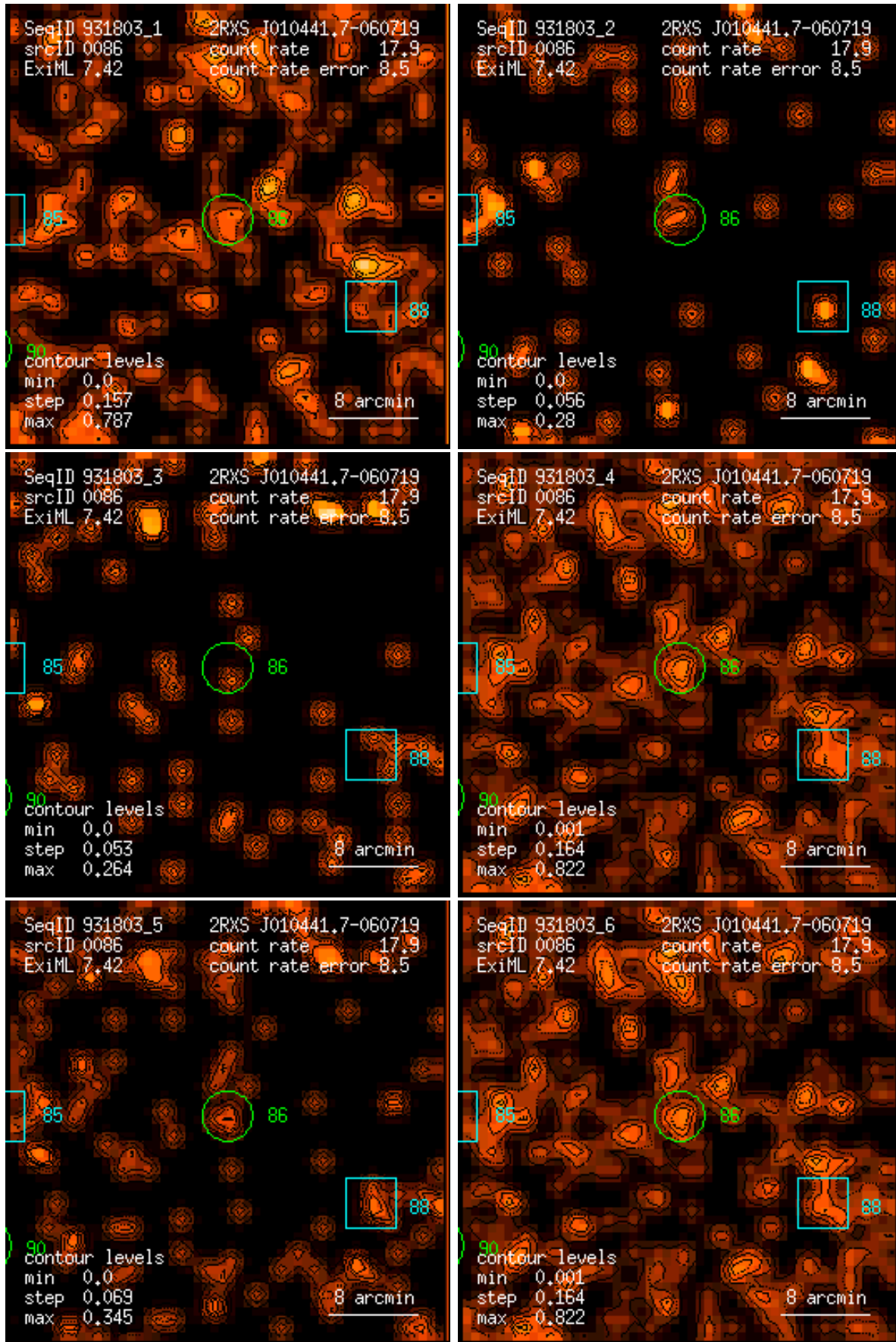
Figure 86: RASS 931803: detection 0086: band rate images, Gaussian filter: (1) PSPC channels 11 – 41, (2) 52 – 90, (3) 91 – 201, (4) 11 – 235, (5) 52 – 201, (6) 11 – 201. Broad band rates in counts/ks. Band rate contour levels in counts/ks/arcmin 2 .
