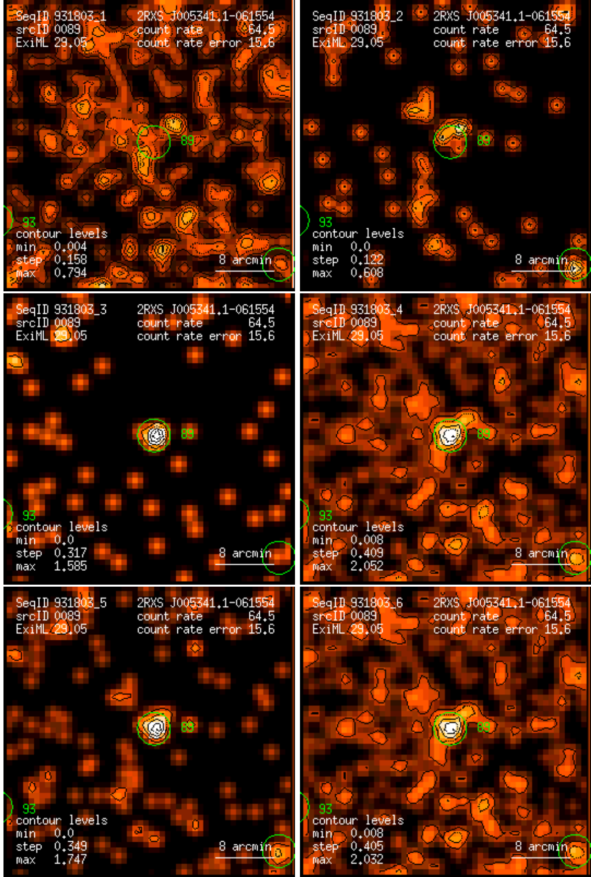
Figure 89: RASS 931803: detection 0089: band rate images, Gaussian filter: (1) PSPC channels 11 – 41, (2) 52 – 90, (3) 91 – 201, (4) 11 – 235, (5) 52 – 201, (6) 11 – 201. Broad band rates in counts/ks. Band rate contour levels in counts/ks/arcmin 2 .
