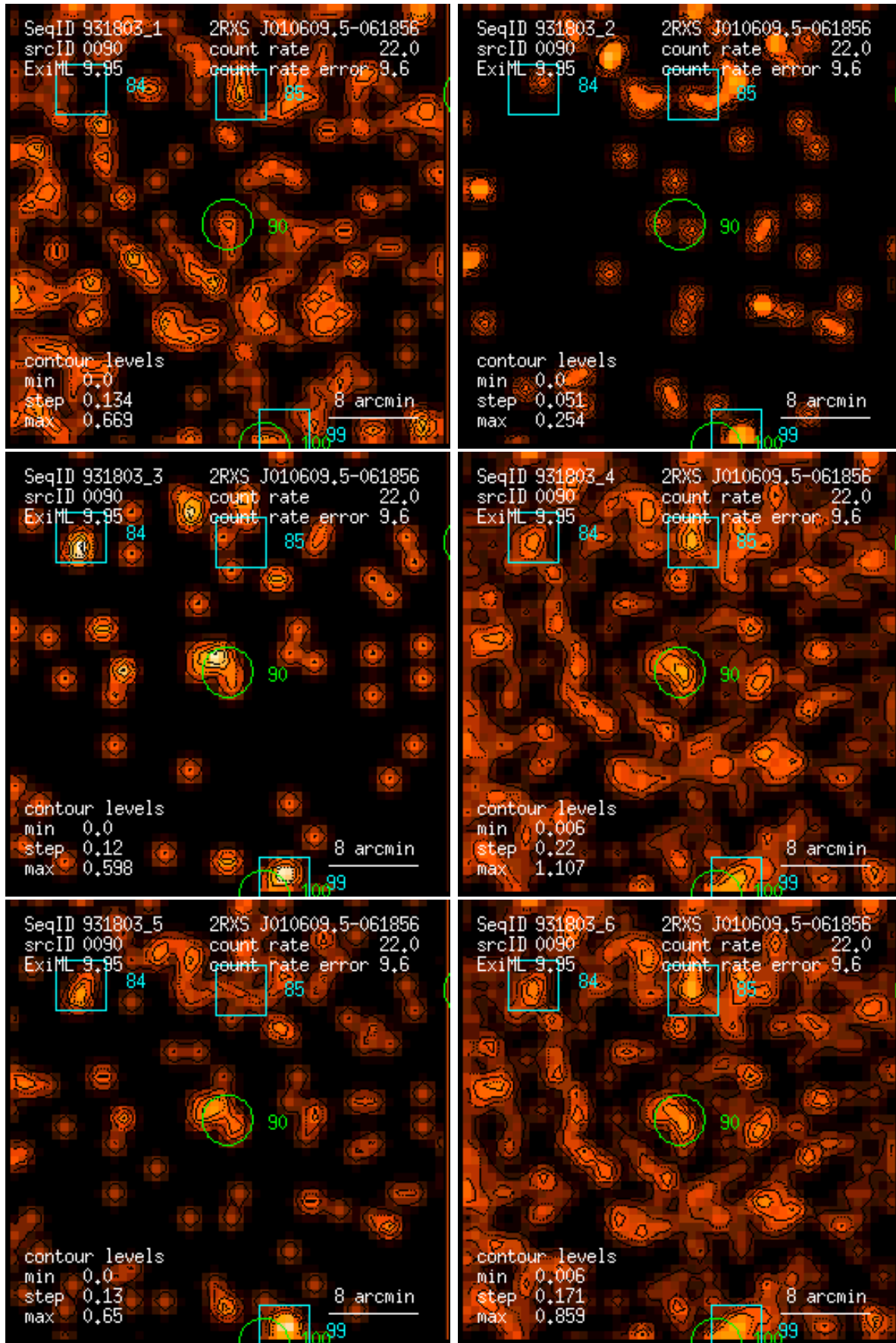
Figure 90: RASS 931803: detection 0090: band rate images, Gaussian filter: (1) PSPC channels 11 – 41, (2) 52 – 90, (3) 91 – 201, (4) 11 – 235, (5) 52 – 201, (6) 11 – 201. Broad band rates in counts/ks. Band rate contour levels in counts/ks/arcmin 2 .
