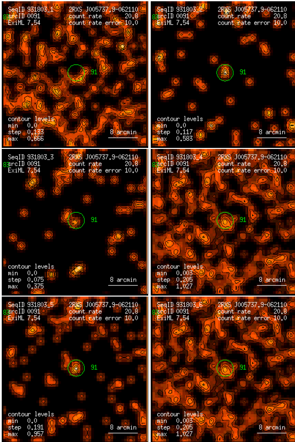
Figure 91: RASS 931803: detection 0091: band rate images, Gaussian filter: (1) PSPC channels 11 – 41, (2) 52 – 90, (3) 91 – 201, (4) 11 – 235, (5) 52 – 201, (6) 11 – 201. Broad band rates in counts/ks. Band rate contour levels in counts/ks/arcmin 2 .
