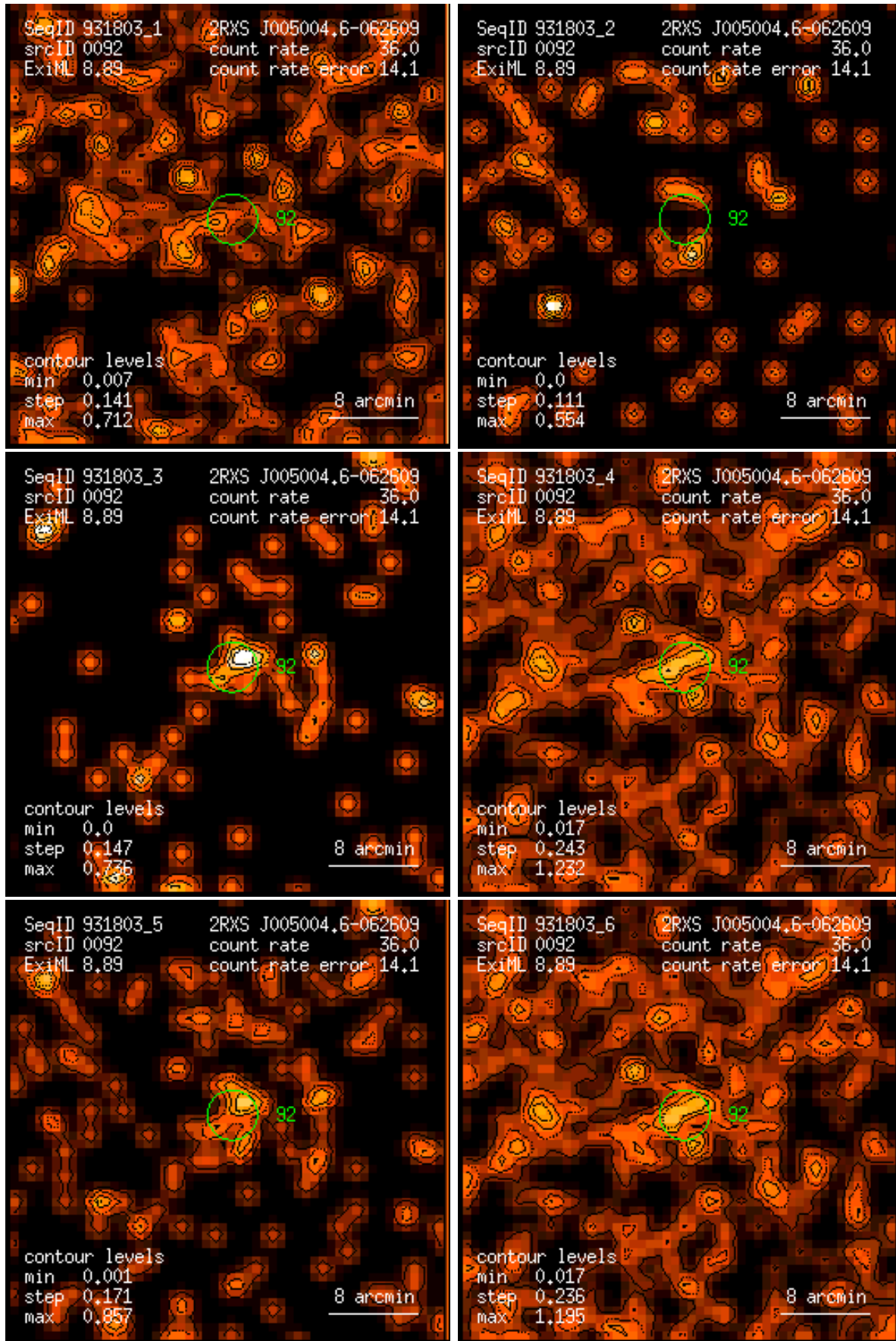
Figure 92: RASS 931803: detection 0092: band rate images, Gaussian filter: (1) PSPC channels 11 – 41, (2) 52 – 90, (3) 91 – 201, (4) 11 – 235, (5) 52 – 201, (6) 11 – 201. Broad band rates in counts/ks. Band rate contour levels in counts/ks/arcmin 2 .
