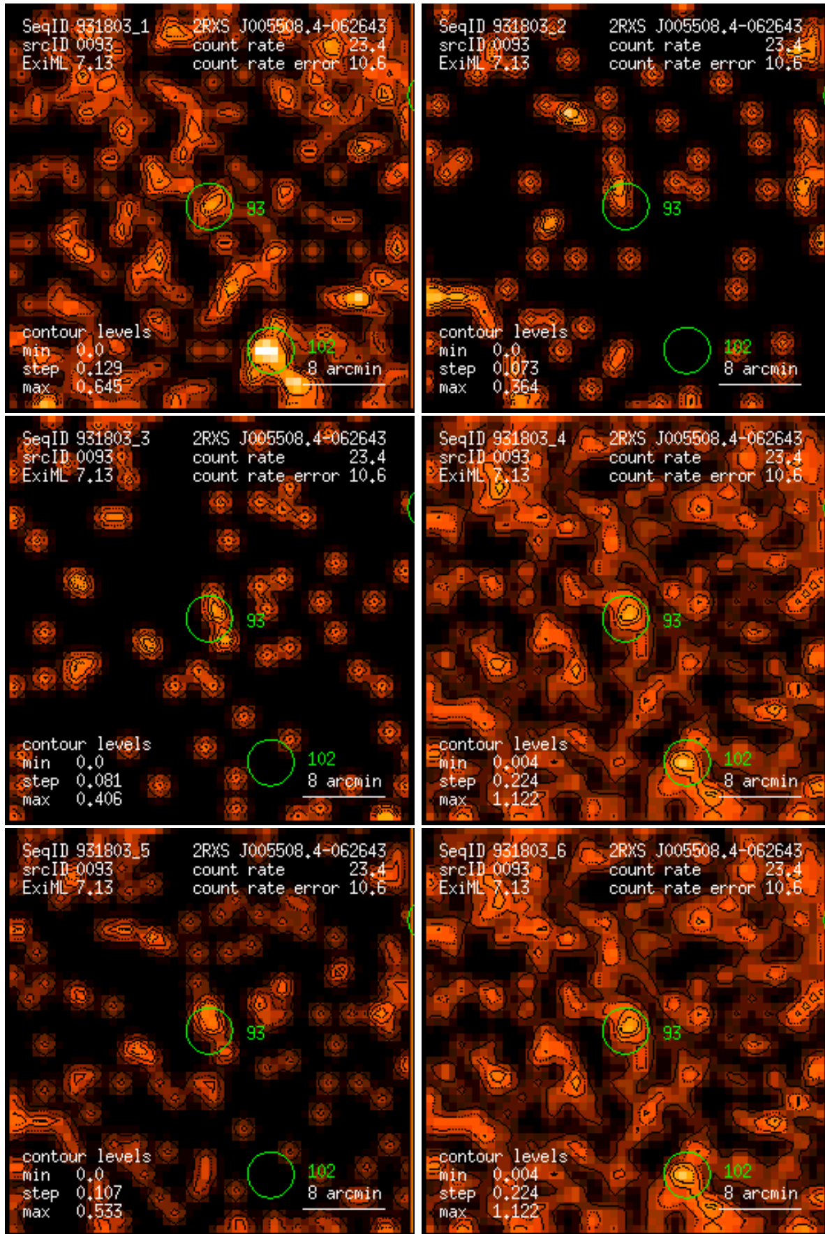
Figure 93: RASS 931803: detection 0093: band rate images, Gaussian filter: (1) PSPC channels 11 – 41, (2) 52 – 90, (3) 91 – 201, (4) 11 – 235, (5) 52 – 201, (6) 11 – 201. Broad band rates in counts/ks. Band rate contour levels in counts/ks/arcmin 2 .
