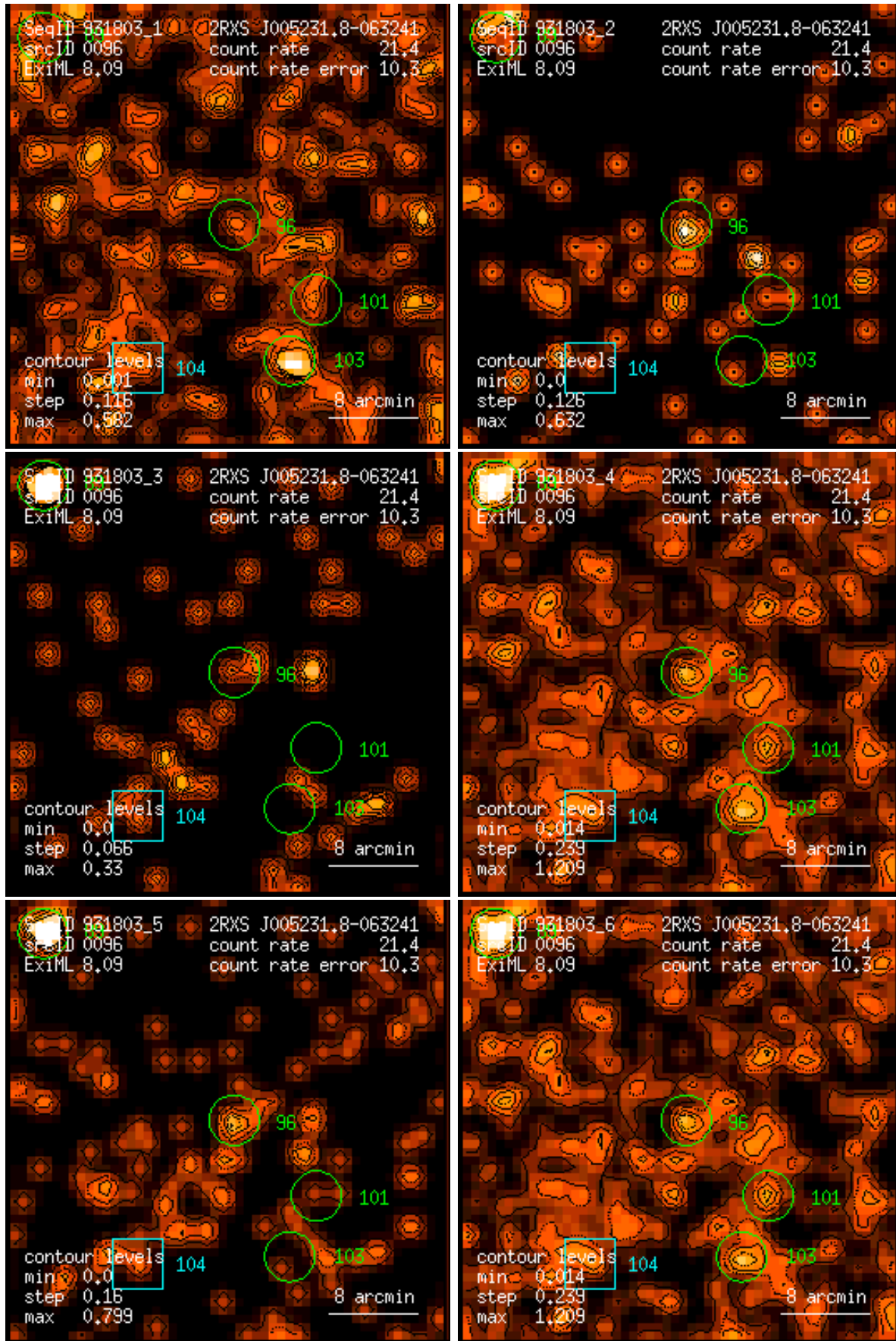
Figure 96: RASS 931803: detection 0096: band rate images, Gaussian filter: (1) PSPC channels 11 – 41, (2) 52 – 90, (3) 91 – 201, (4) 11 – 235, (5) 52 – 201, (6) 11 – 201. Broad band rates in counts/ks. Band rate contour levels in counts/ks/arcmin 2 .
