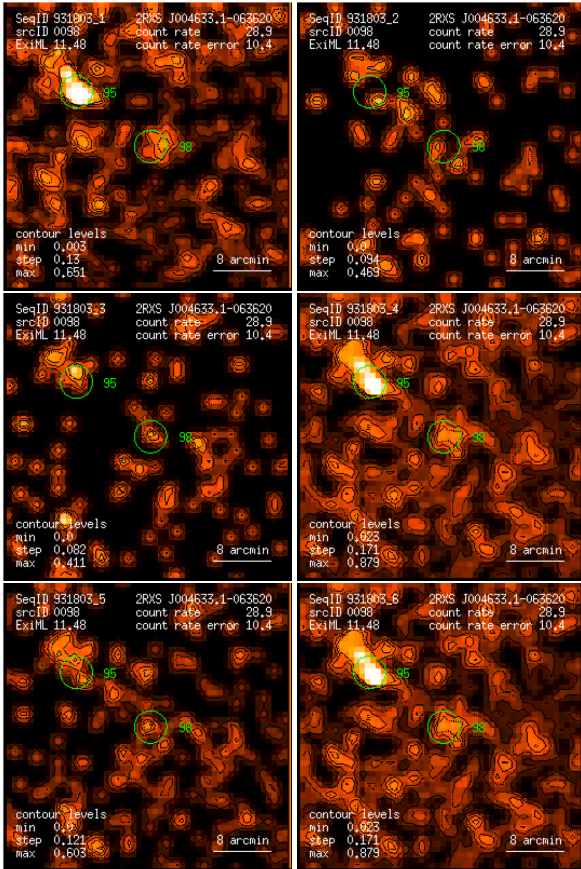
Figure 98: RASS 931803: detection 0098: band rate images, Gaussian filter: (1) PSPC channels 11 – 41, (2) 52 – 90, (3) 91 – 201, (4) 11 – 235, (5) 52 – 201, (6) 11 – 201. Broad band rates in counts/ks. Band rate contour levels in counts/ks/arcmin 2 .
