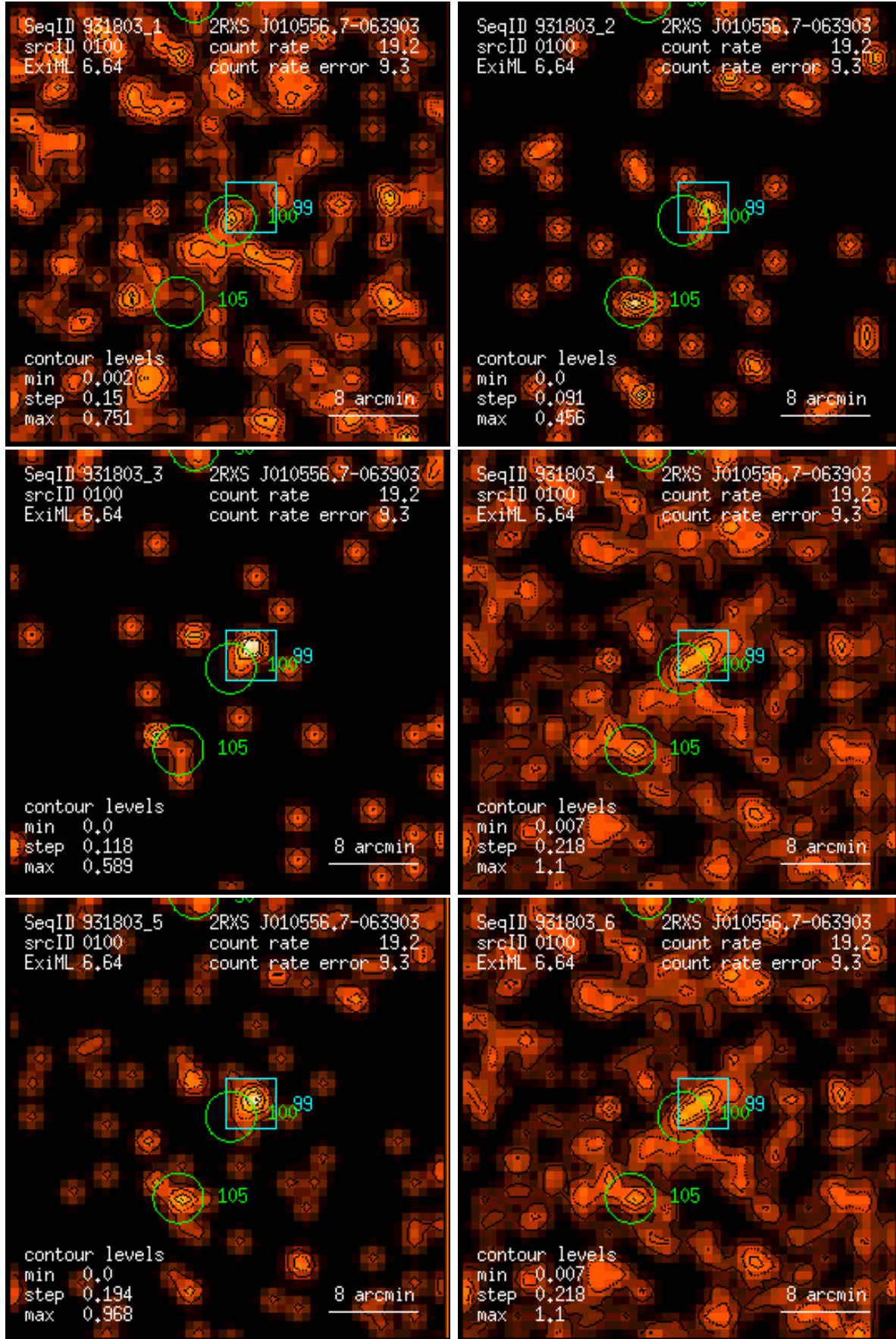
Figure 100: RASS 931803: detection 0100: band rate images, Gaussian filter: (1) PSPC channels 11 – 41, (2) 52 – 90, (3) 91 – 201, (4) 11 – 235, (5) 52 – 201, (6) 11 – 201. Broad band rates in counts/ks. Band rate contour levels in counts/ks/arcmin 2 .
