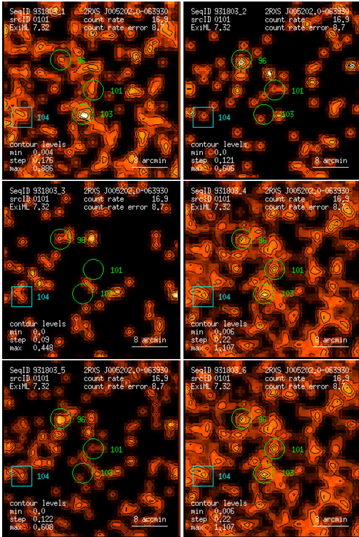
Figure 101: RASS 931803: detection 0101: band rate images, Gaussian filter: (1) PSPC channels 11 – 41, (2) 52 – 90, (3) 91 – 201, (4) 11 – 235, (5) 52 – 201, (6) 11 – 201. Broad band rates in counts/ks. Band rate contour levels in counts/ks/arcmin 2 .
