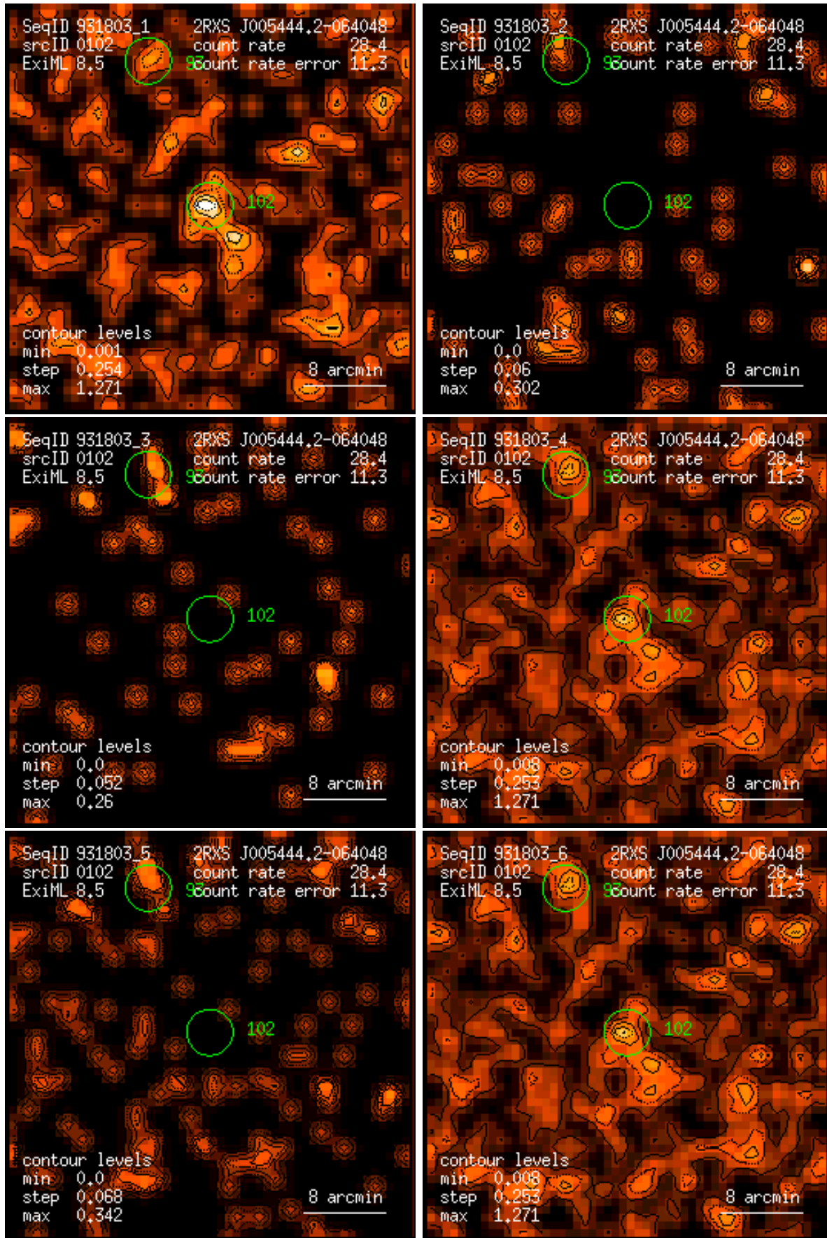
Figure 102: RASS 931803: detection 0102: band rate images, Gaussian filter: (1) PSPC channels 11 – 41, (2) 52 – 90, (3) 91 – 201, (4) 11 – 235, (5) 52 – 201, (6) 11 – 201. Broad band rates in counts/ks. Band rate contour levels in counts/ks/arcmin 2 .
