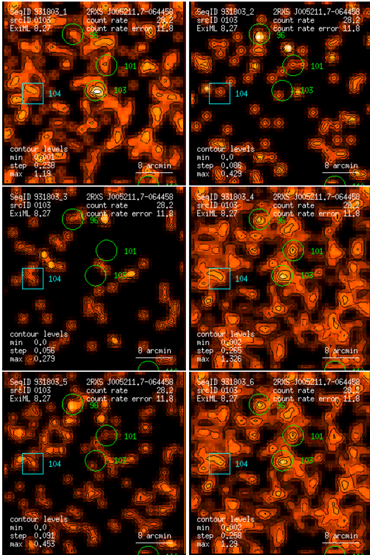
Figure 103: RASS 931803: detection 0103: band rate images, Gaussian filter: (1) PSPC channels 11 – 41, (2) 52 – 90, (3) 91 – 201, (4) 11 – 235, (5) 52 – 201, (6) 11 – 201. Broad band rates in counts/ks. Band rate contour levels in counts/ks/arcmin 2 .
