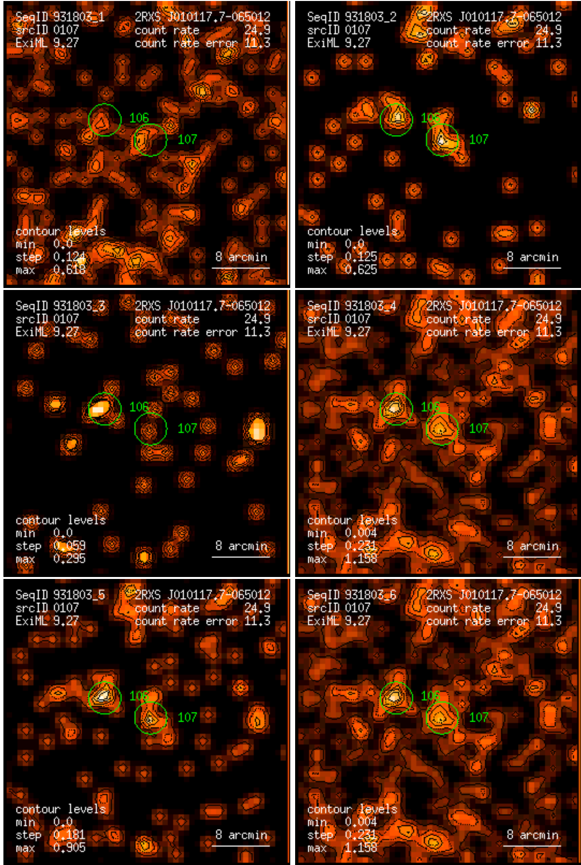
Figure 107: RASS 931803: detection 0107: band rate images, Gaussian filter: (1) PSPC channels 11 – 41, (2) 52 – 90, (3) 91 – 201, (4) 11 – 235, (5) 52 – 201, (6) 11 – 201. Broad band rates in counts/ks. Band rate contour levels in counts/ks/arcmin 2 .
