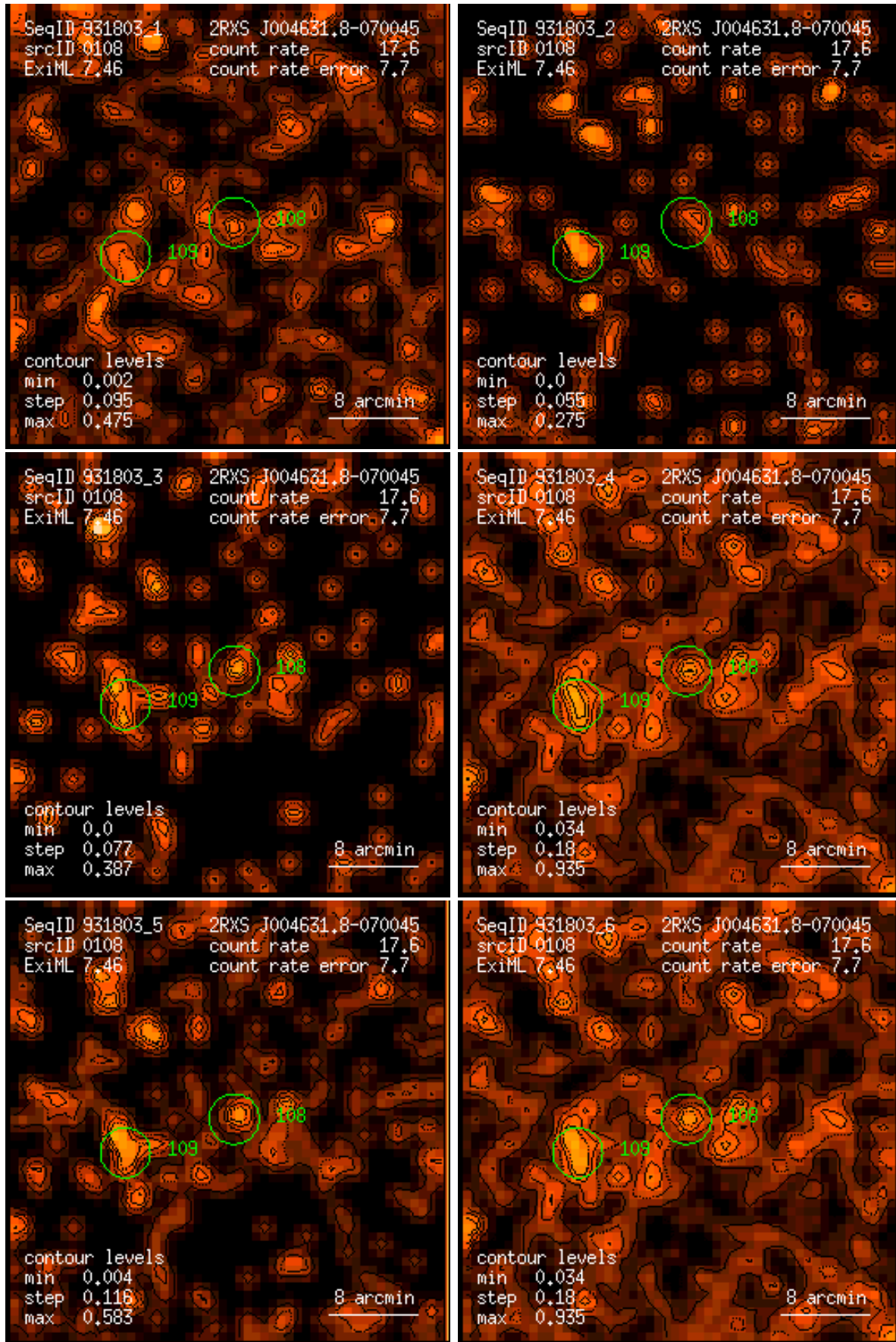
Figure 108: RASS 931803: detection 0108: band rate images, Gaussian filter: (1) PSPC channels 11 – 41, (2) 52 – 90, (3) 91 – 201, (4) 11 – 235, (5) 52 – 201, (6) 11 – 201. Broad band rates in counts/ks. Band rate contour levels in counts/ks/arcmin 2 .
