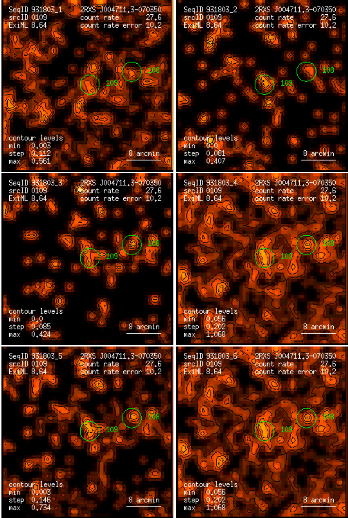
Figure 109: RASS 931803: detection 0109: band rate images, Gaussian filter: (1) PSPC channels 11 – 41, (2) 52 – 90, (3) 91 – 201, (4) 11 – 235, (5) 52 – 201, (6) 11 – 201. Broad band rates in counts/ks. Band rate contour levels in counts/ks/arcmin 2 .
