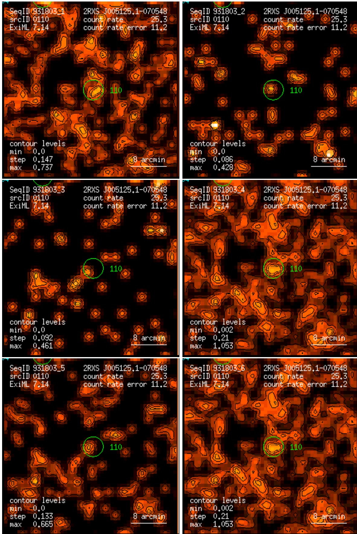
Figure 110: RASS 931803: detection 0110: band rate images, Gaussian filter: (1) PSPC channels 11 – 41, (2) 52 – 90, (3) 91 – 201, (4) 11 – 235, (5) 52 – 201, (6) 11 – 201. Broad band rates in counts/ks. Band rate contour levels in counts/ks/arcmin 2 .
