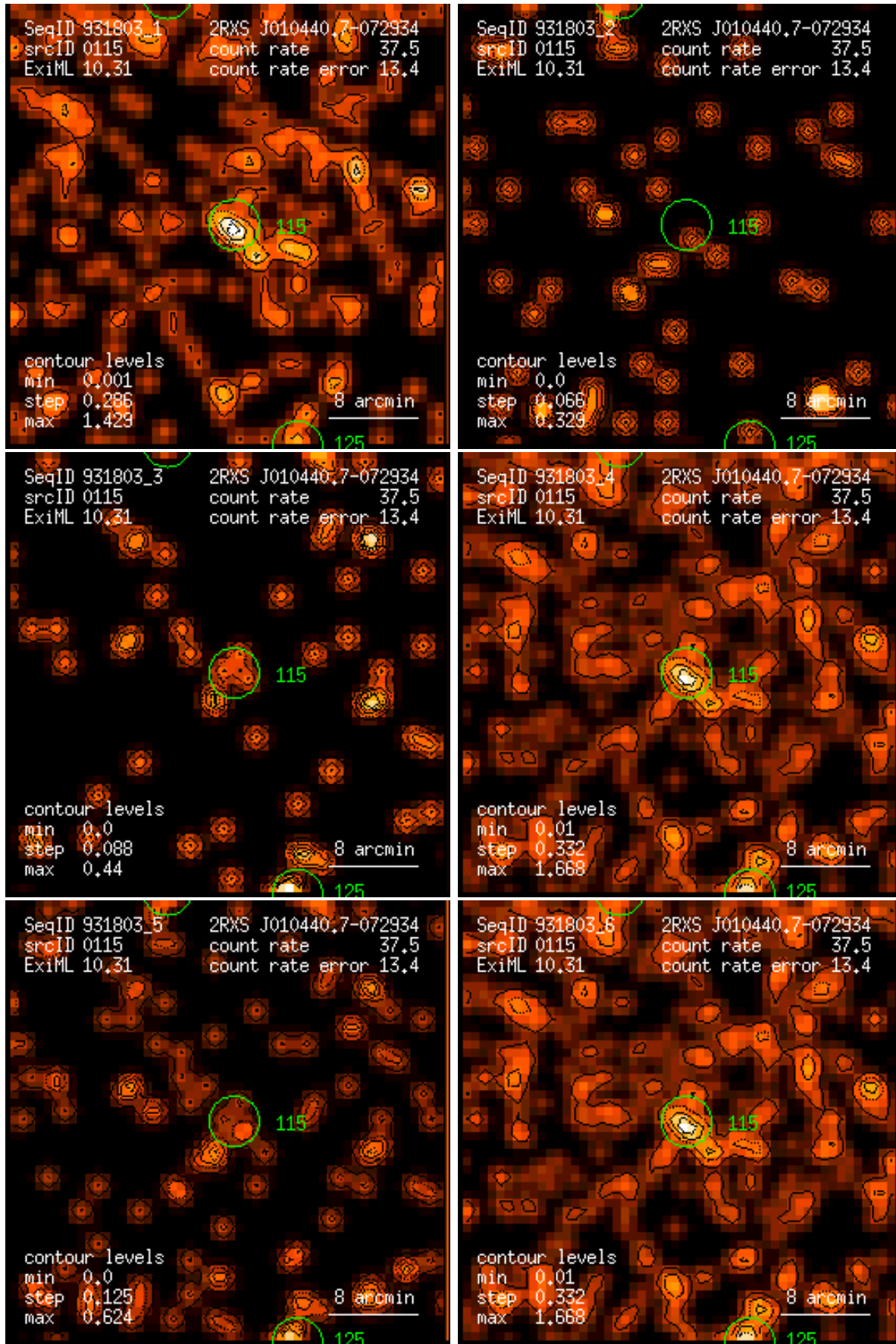
Figure 115: RASS 931803: detection 0115: band rate images, Gaussian filter: (1) PSPC channels 11 – 41, (2) 52 – 90, (3) 91 – 201, (4) 11 – 235, (5) 52 – 201, (6) 11 – 201. Broad band rates in counts/ks. Band rate contour levels in counts/ks/arcmin 2 .
