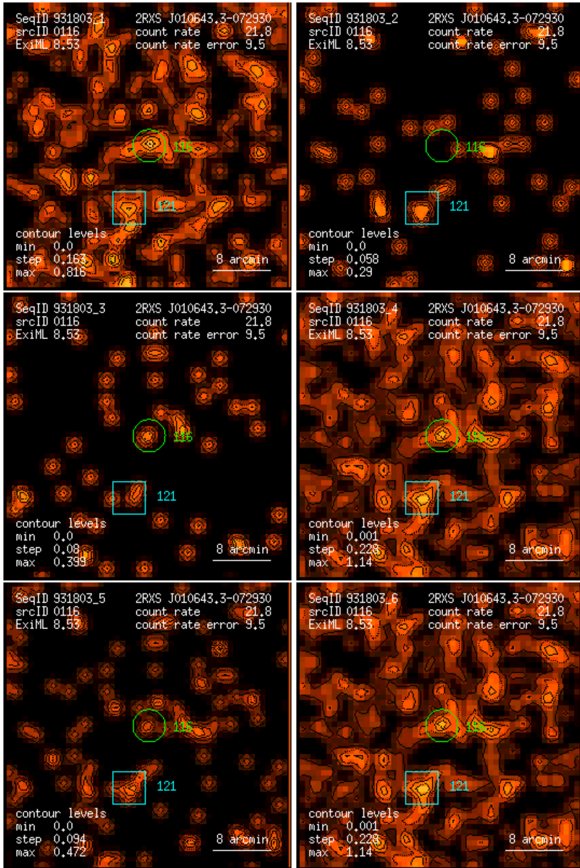
Figure 116: RASS 931803: detection 0116: band rate images, Gaussian filter: (1) PSPC channels 11 – 41, (2) 52 – 90, (3) 91 – 201, (4) 11 – 235, (5) 52 – 201, (6) 11 – 201. Broad band rates in counts/ks. Band rate contour levels in counts/ks/arcmin 2 .
