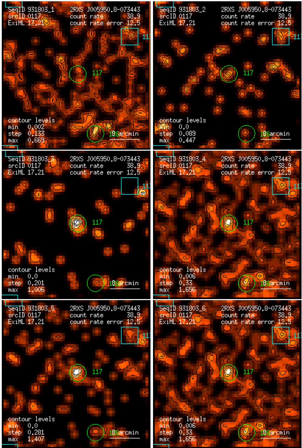
Figure 117: RASS 931803: detection 0117: band rate images, Gaussian filter: (1) PSPC channels 11 – 41, (2) 52 – 90, (3) 91 – 201, (4) 11 – 235, (5) 52 – 201, (6) 11 – 201. Broad band rates in counts/ks. Band rate contour levels in counts/ks/arcmin 2 .
