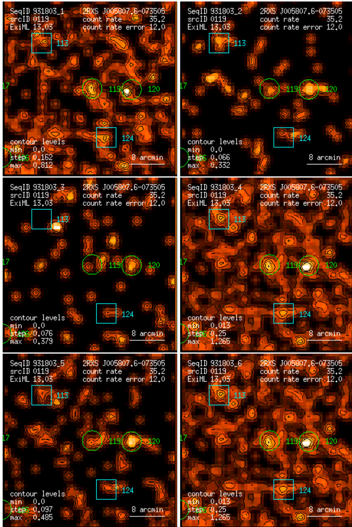
Figure 119: RASS 931803: detection 0119: band rate images, Gaussian filter: (1) PSPC channels 11 – 41, (2) 52 – 90, (3) 91 – 201, (4) 11 – 235, (5) 52 – 201, (6) 11 – 201. Broad band rates in counts/ks. Band rate contour levels in counts/ks/arcmin 2 .
