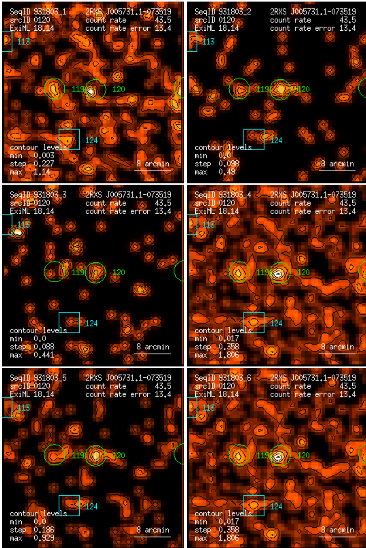
Figure 120: RASS 931803: detection 0120: band rate images, Gaussian filter: (1) PSPC channels 11 – 41, (2) 52 – 90, (3) 91 – 201, (4) 11 – 235, (5) 52 – 201, (6) 11 – 201. Broad band rates in counts/ks. Band rate contour levels in counts/ks/arcmin 2 .
